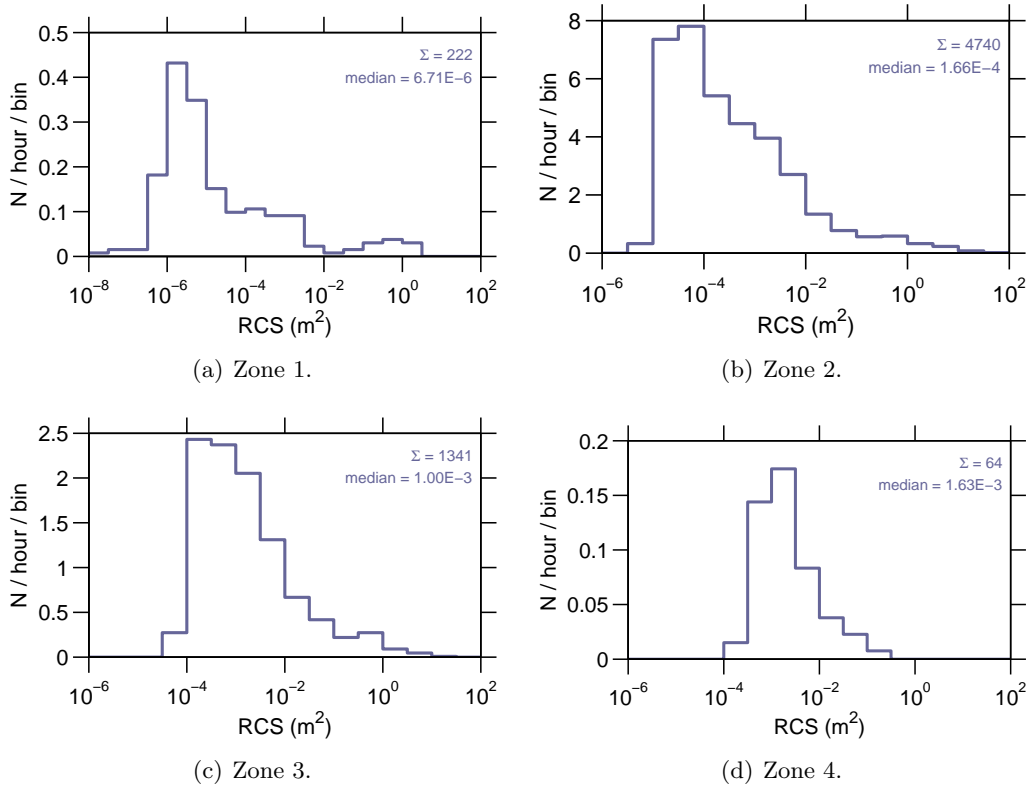
Figure 9: Event rate v radar cross section, 04 Feb–10 Feb 2008.
