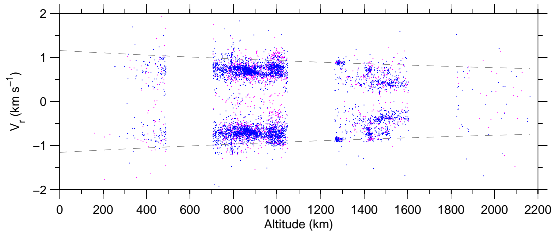
Figure 7: Doppler-velocity v altitude , 04 Feb–10 Feb 2008.
