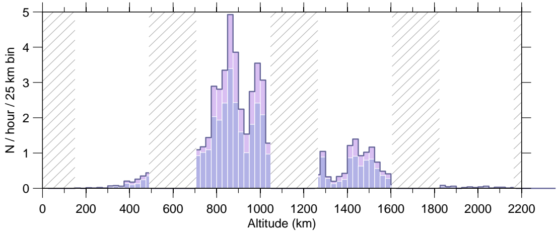
Figure 6: Event rate v altitude , 04 Feb–10 Feb 2008.
