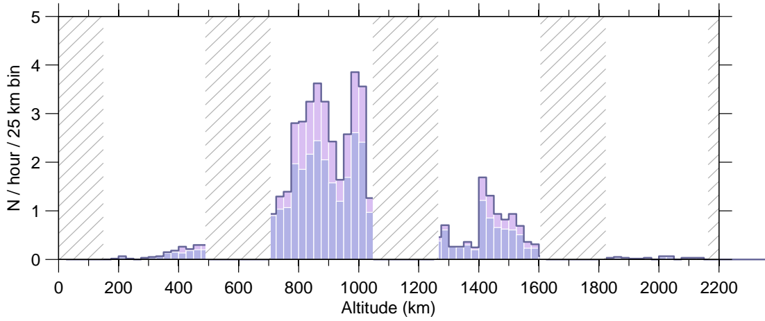
Figure 6: Event rate v altitude , 28 Jan–03 Feb 2008.
