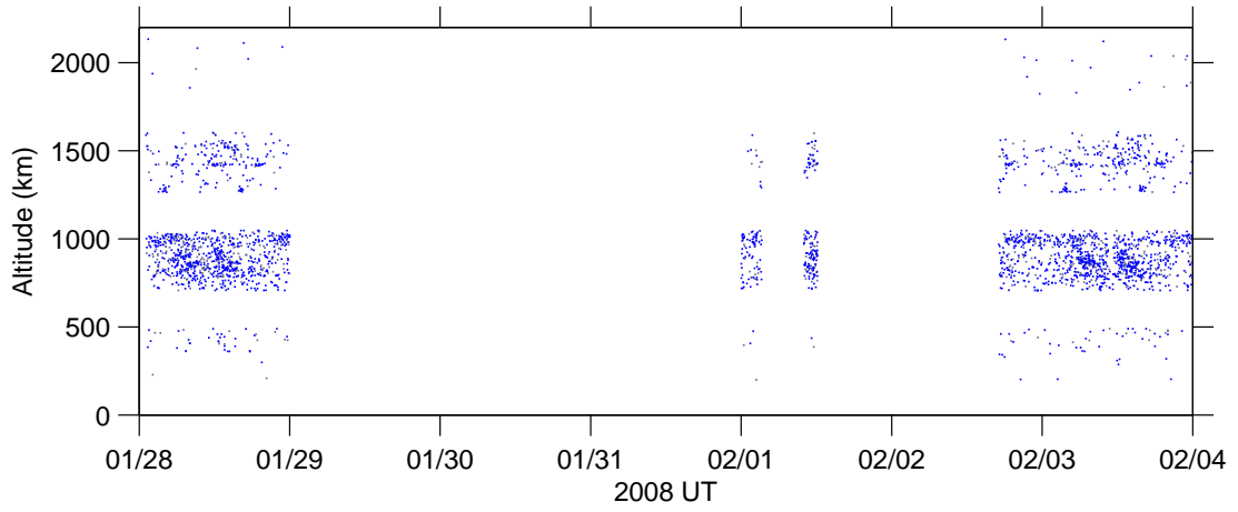
Figure 5: Altitude v time , 28 Jan–03 Feb 2008.
