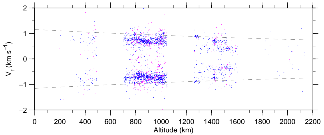
Figure 7: Doppler-velocity v altitude , 28 Jan–03 Feb 2008.
