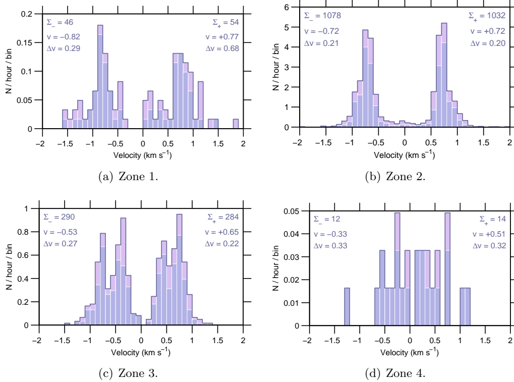
Figure 8: Event rate v Doppler-velocity , 28 Jan–03 Feb 2008.
