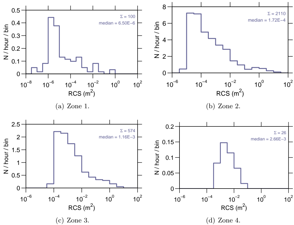
Figure 9: Event rate v radar cross section , 28 Jan–03 Feb 2008.
