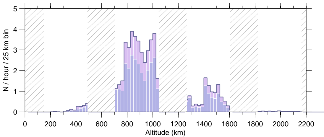
Figure 6: Event rate v altitude , 21 Jan–27 Jan 2008.
