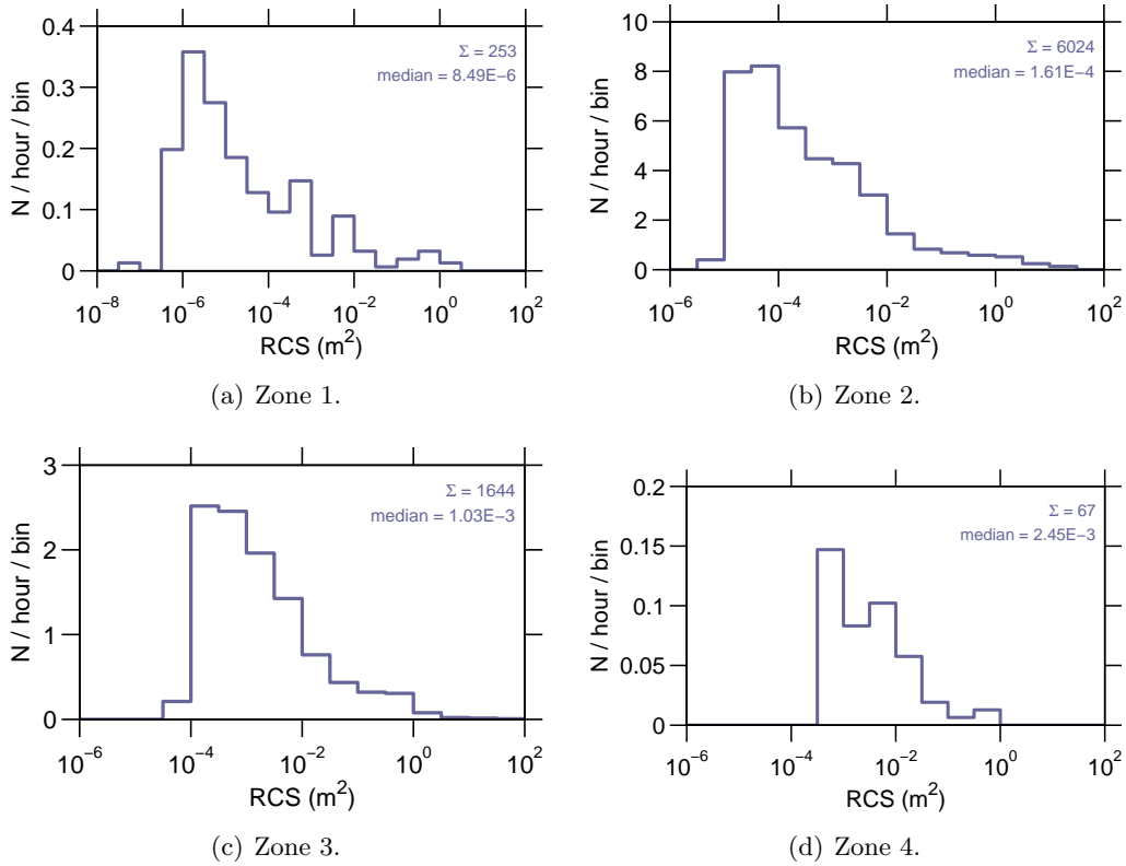
Figure 9: Event rate v radar cross section , 21 Jan–27 Jan 2008.
