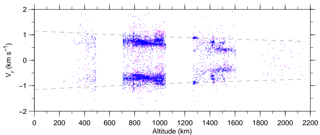
Figure 7: Doppler-velocity v altitude , 21 Jan–27 Jan 2008.
