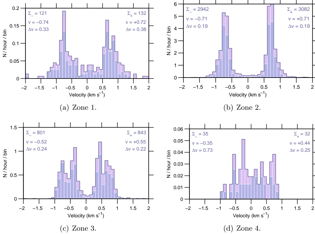
Figure 8: Event rate v Doppler-velocity , 21 Jan–27 Jan 2008.
