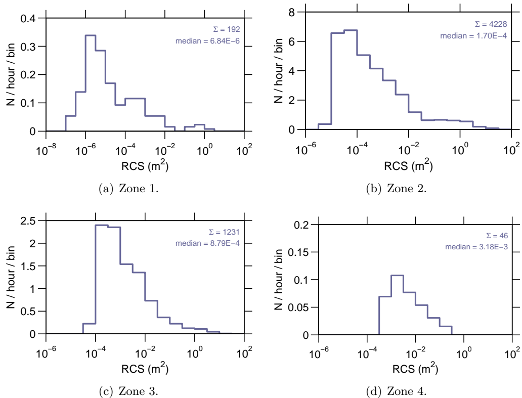
Figure 9: Event rate v radar cross section , 14 Jan–20 Jan 2008.
