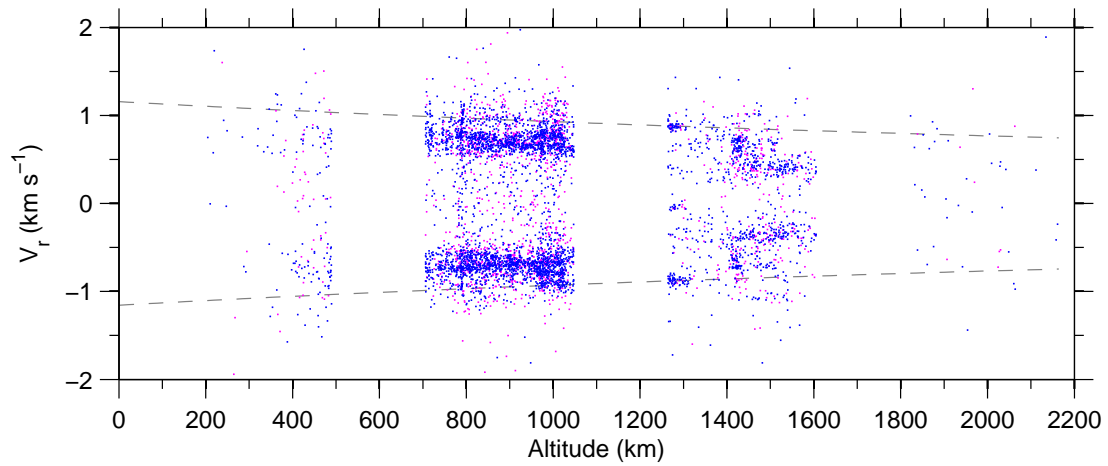
Figure 7: Doppler-velocity v altitude , 14 Jan–20 Jan 2008.
