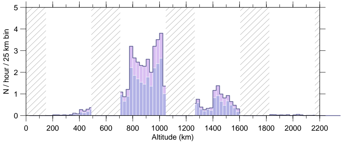
Figure 6: Event rate v altitude , 14 Jan–20 Jan 2008.
