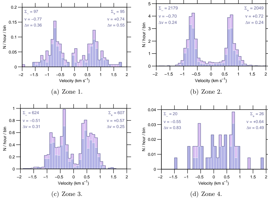
Figure 8: Event rate v Doppler-velocity , 14 Jan–20 Jan 2008.
