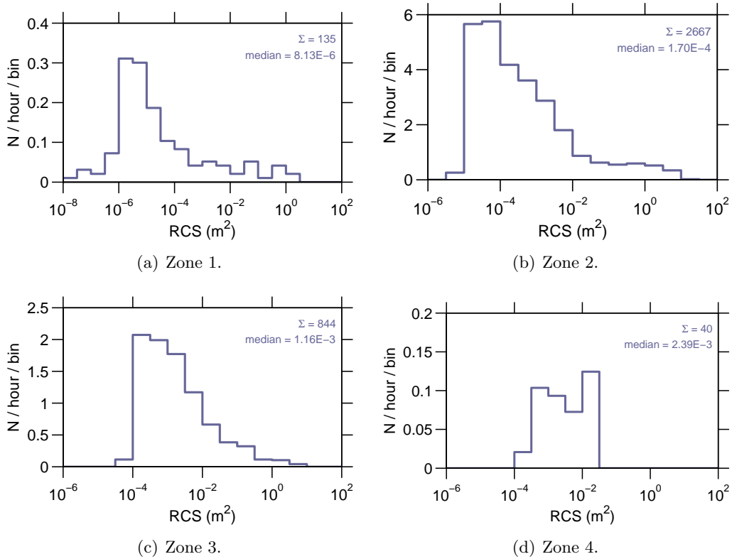
Figure 9: Event rate v radar cross section, 07 Jan–13 Jan 2008.
