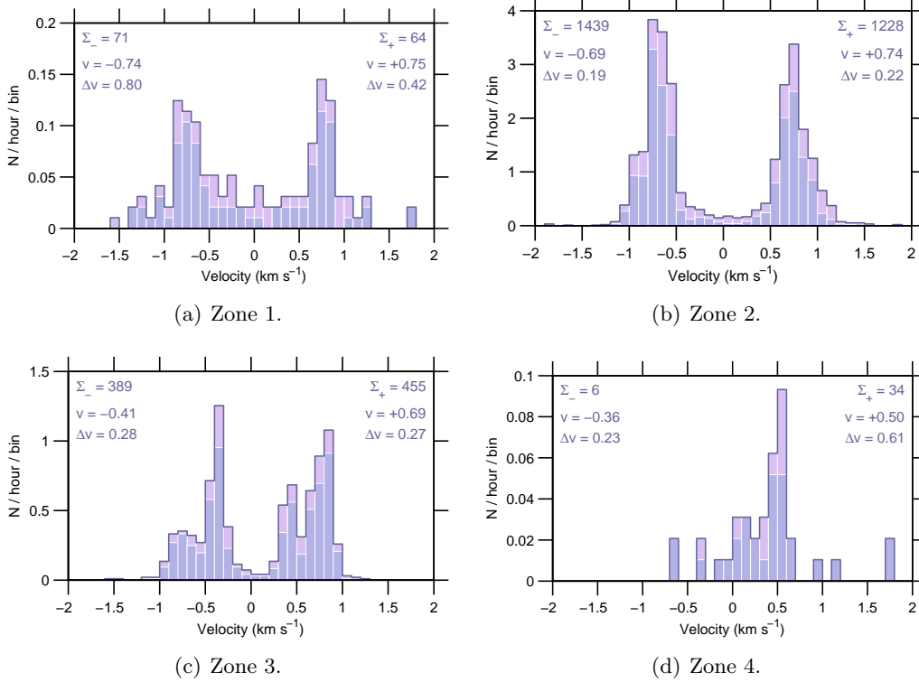
Figure 8: Event rate v Doppler-velocity, 07 Jan–13 Jan 2008.
