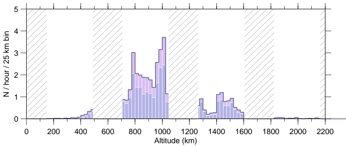
Figure 6: Event rate v altitude , 07 Jan–13 Jan 2008.
