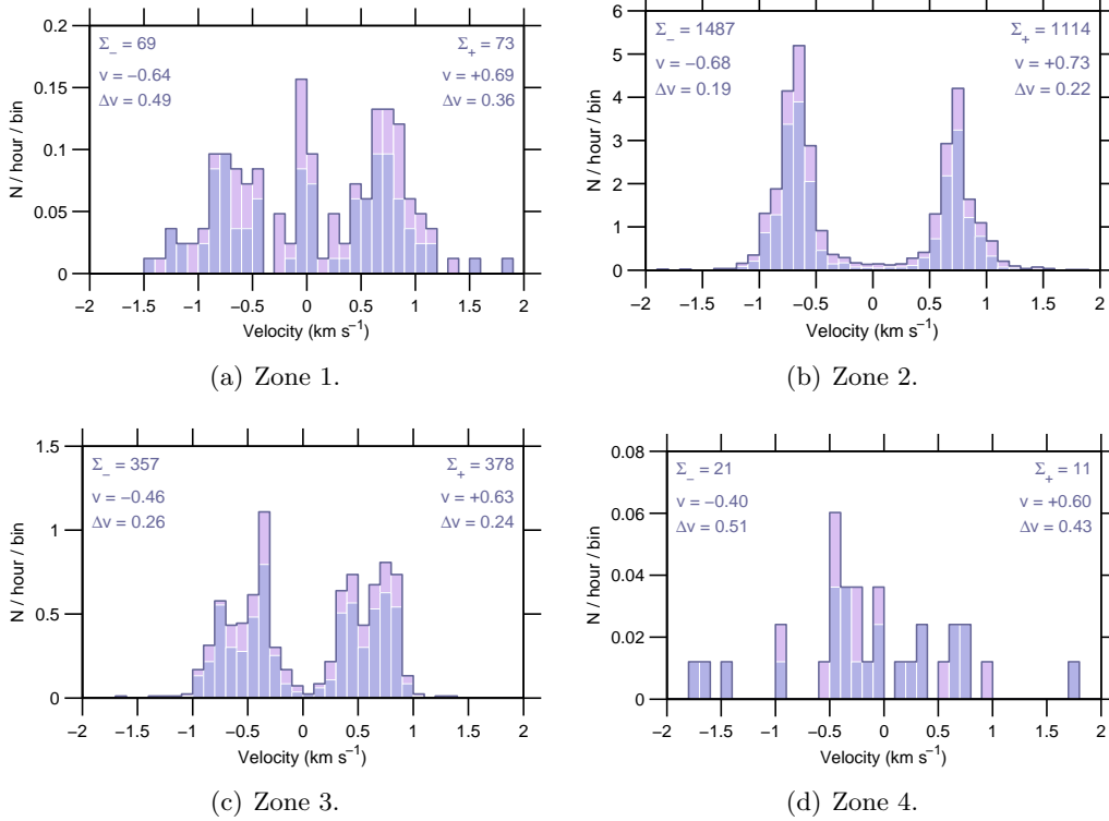
Figure 8: Event rate v Doppler-velocity , 31 Dec-06 Jan 2007.
