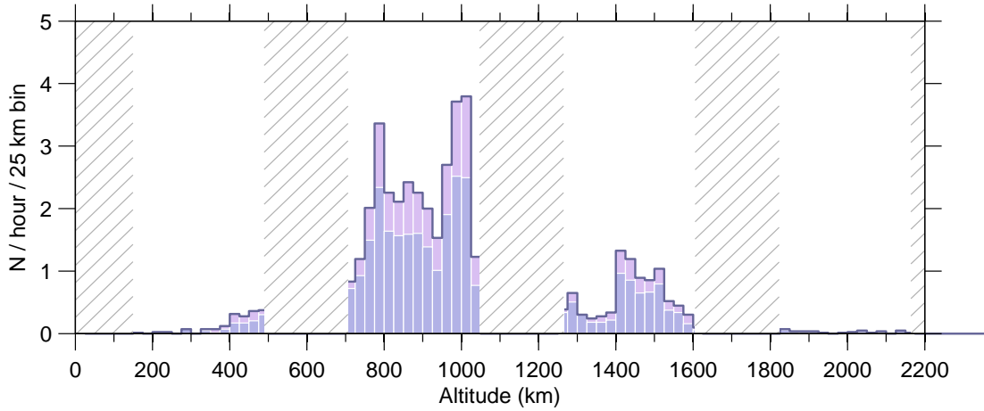
Figure 6: Event rate v altitude , 31 Dec–06 Jan 2007.
