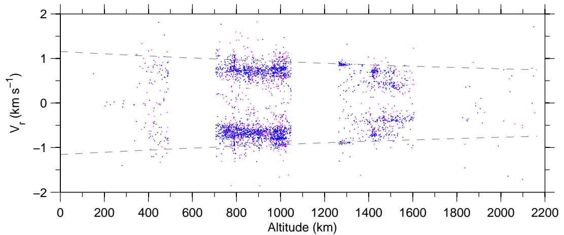
Figure 7: Doppler-velocity v altitude , 31 Dec–06 Jan 2007.
