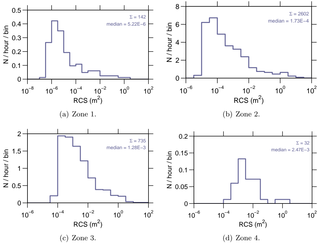
Figure 9: Event rate v radar cross section , 31 Dec-06 Jan 2007.
