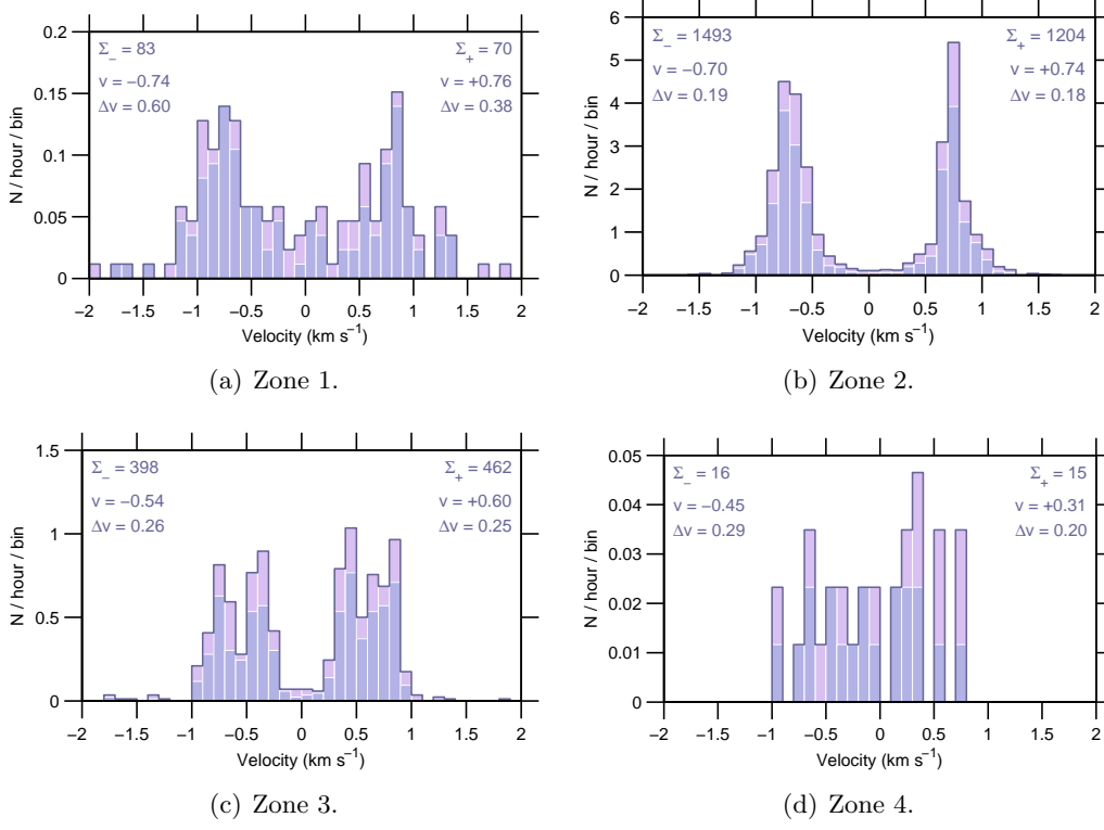
Figure 8: Event rate v Doppler-velocity , 24 Dec–30 Dec 2007.
