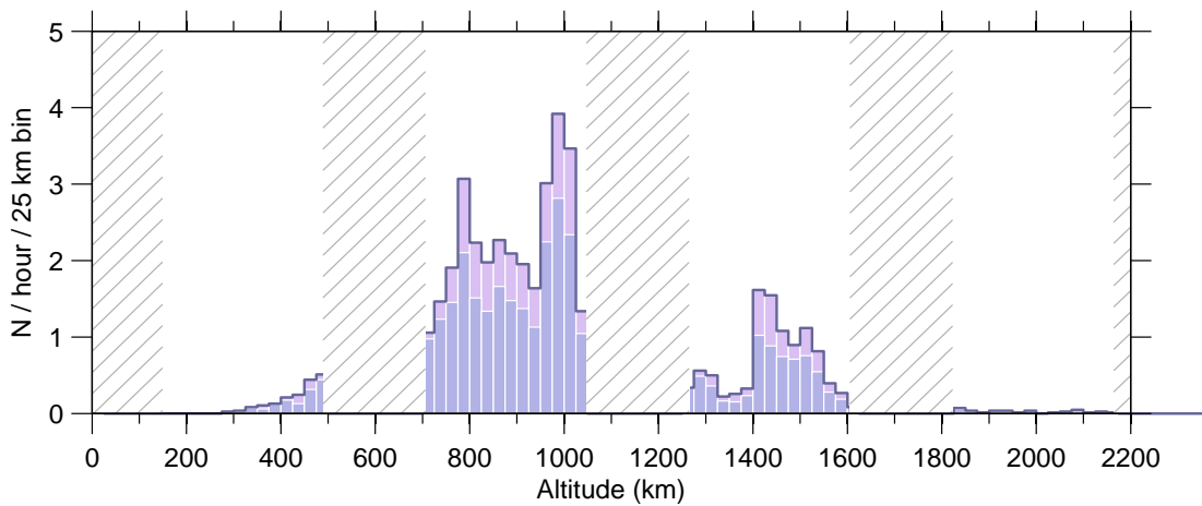
Figure 6: Event rate v altitude, 24 Dec–30 Dec 2007.
