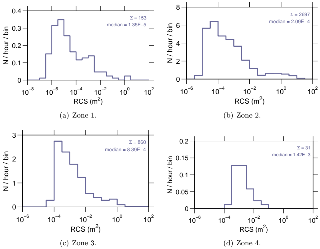
Figure 9: Event rate v radar cross section , 24 Dec–30 Dec 2007.
