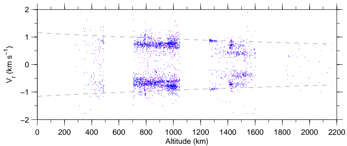
Figure 7: Doppler-velocity v altitude, 24 Dec–30 Dec 2007.
