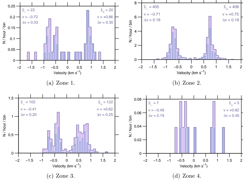
Figure 8: Event rate v Doppler-velocity , 03 Dec–09 Dec 2007.
