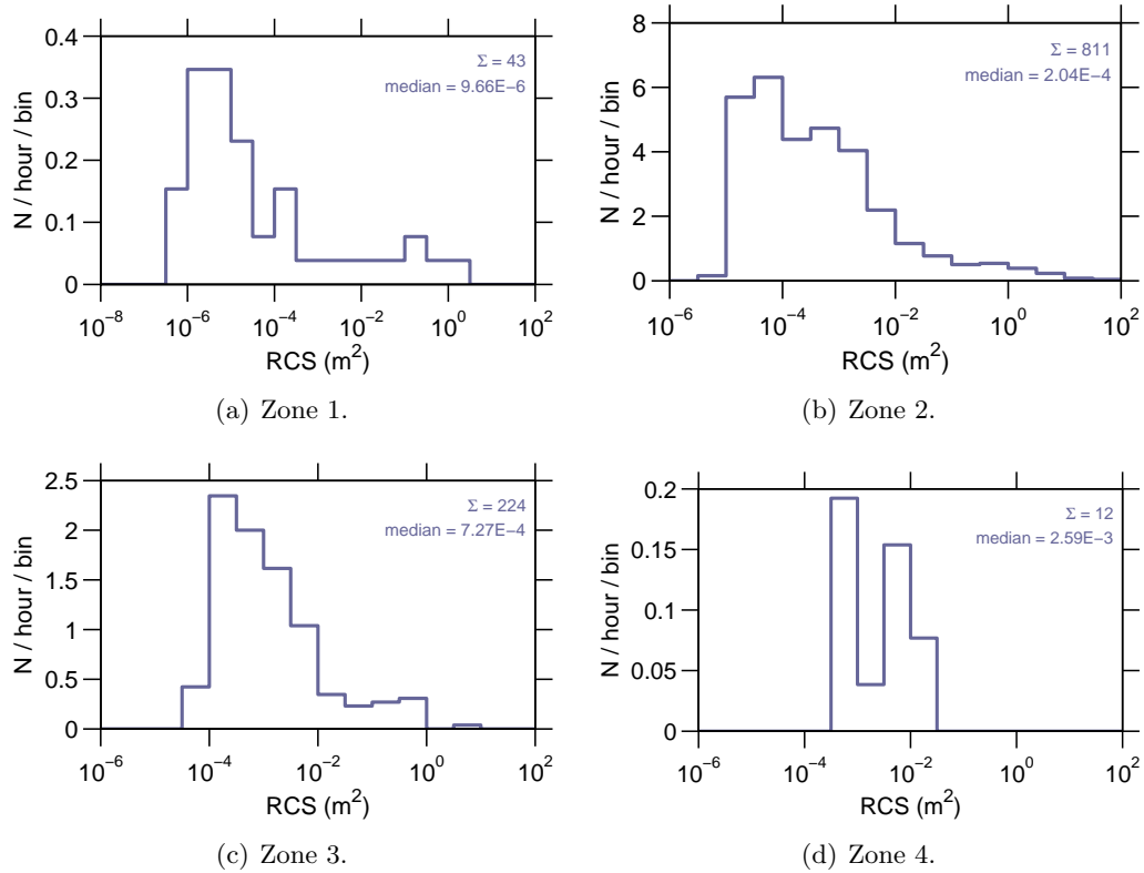
Figure 9: Event rate v radar cross section , 03 Dec–09 Dec 2007.
