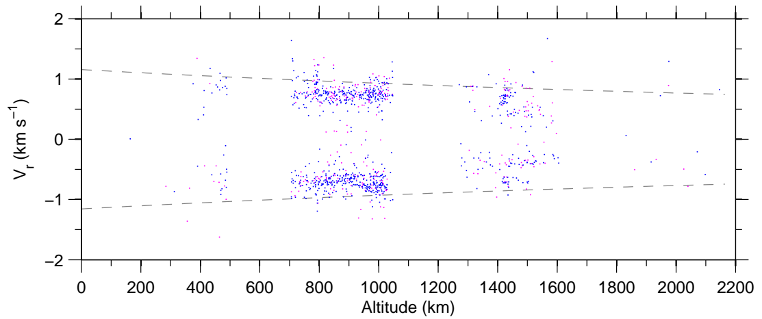
Figure 7: Doppler-velocity v altitude, 03 Dec–09 Dec 2007.
