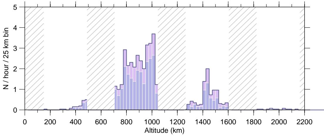
Figure 6: Event rate v altitude, 03 Dec–09 Dec 2007.
