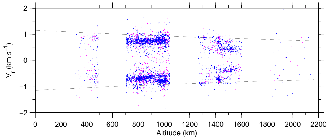
Figure 7: Doppler-velocity v altitude , 26 Nov–02 Dec 2007.
