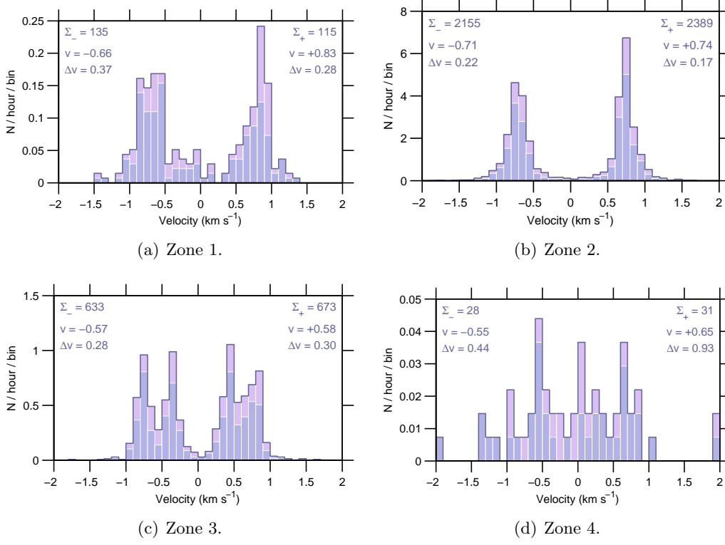
Figure 8: Event rate v Doppler-velocity , 26 Nov–02 Dec 2007.
