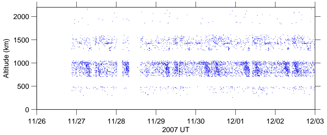
Figure 5: Altitude v time , 26 Nov–02 Dec 2007.
