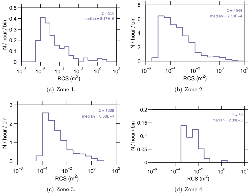
Figure 9: Event rate v radar cross section , 26 Nov–02 Dec 2007.
