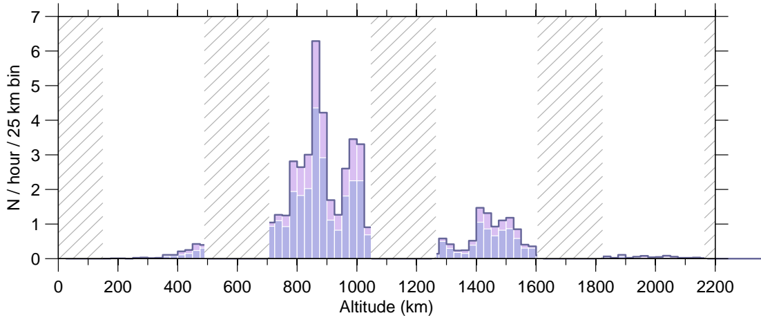
Figure 6: Event rate v altitude, 08 Oct–14 Oct 2007.
