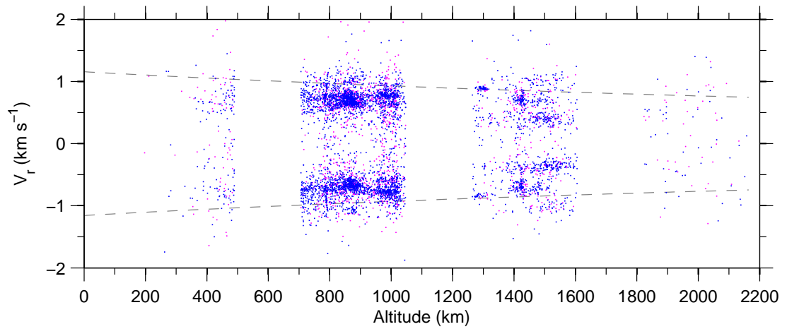
Figure 7: Doppler-velocity v altitude, 08 Oct–14 Oct 2007.
