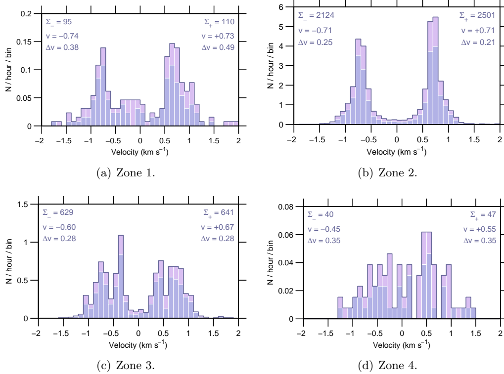
Figure 8: Event rate v Doppler-velocity , 08 Oct–14 Oct 2007.
