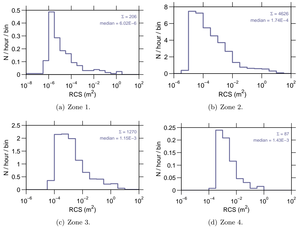
Figure 9: Event rate v radar cross section , 08 Oct–14 Oct 2007.
