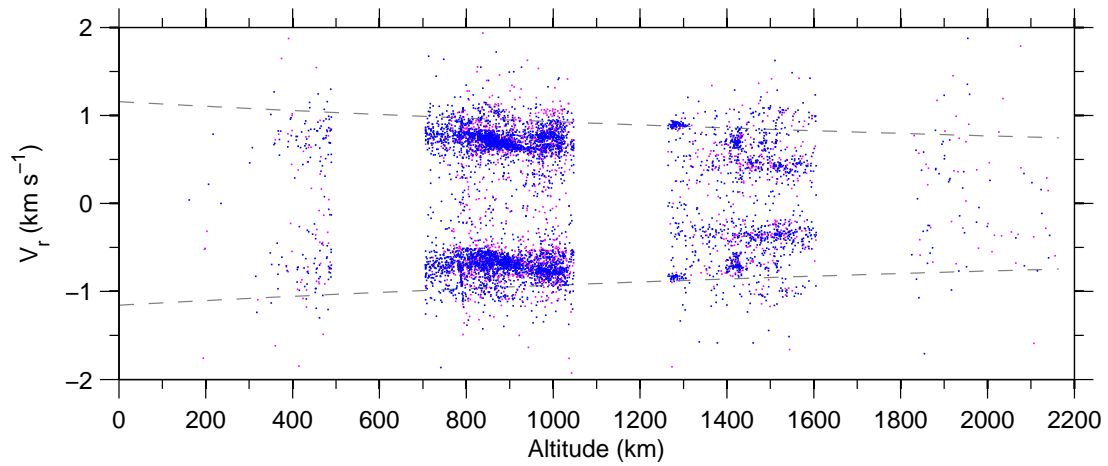
Figure 7: Doppler-velocity v altitude , 24 Sep–30 Sep 2007.
