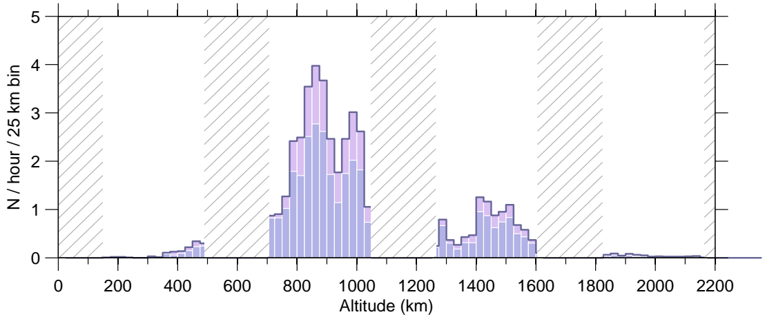
Figure 6: Event rate v altitude , 24 Sep–30 Sep 2007.
