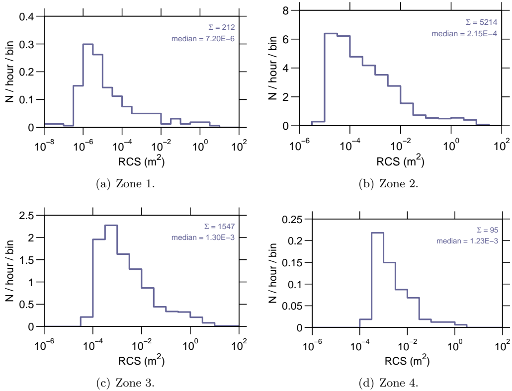
Figure 9: Event rate v radar cross section , 24 Sep–30 Sep 2007.
