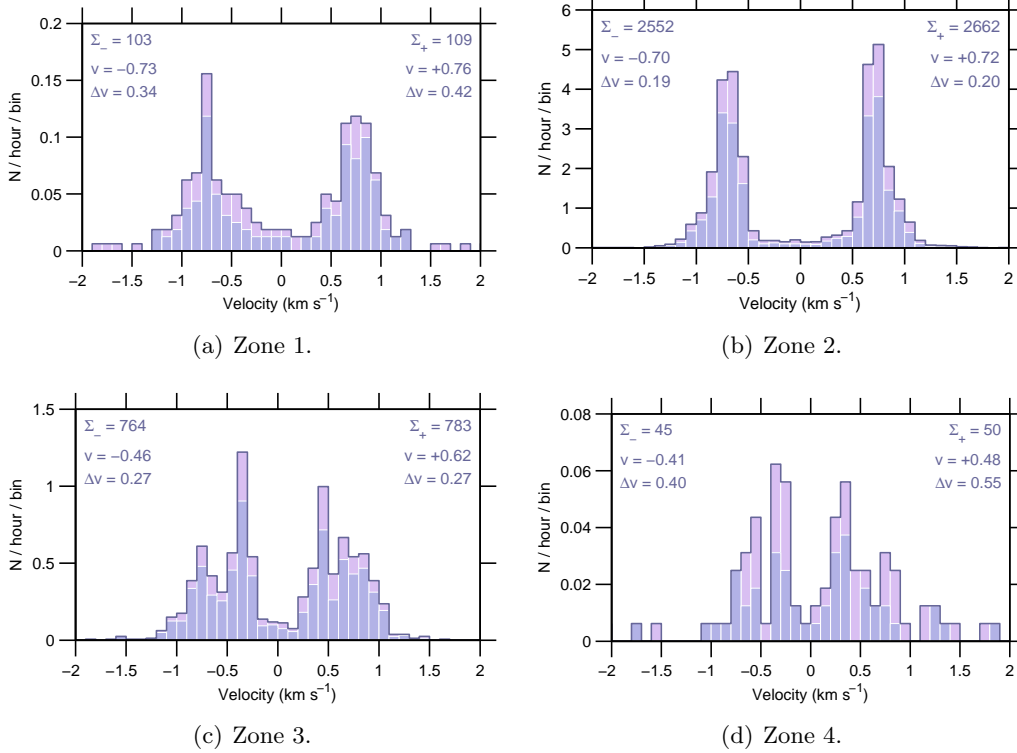
Figure 8: Event rate v Doppler-velocity , 24 Sep–30 Sep 2007.
