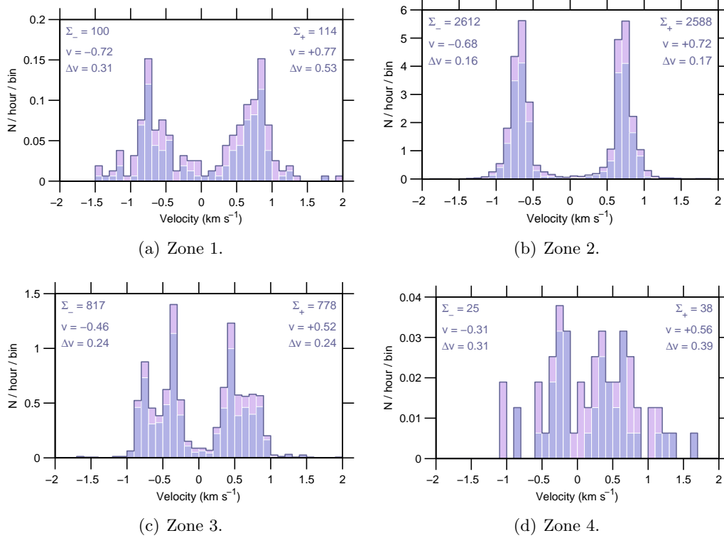
Figure 8: Event rate v Doppler-velocity , 17 Sep–23 Sep 2007.
