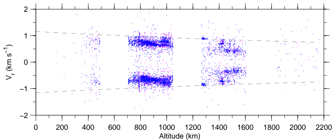
Figure 7: Doppler-velocity v altitude , 17 Sep–23 Sep 2007.
