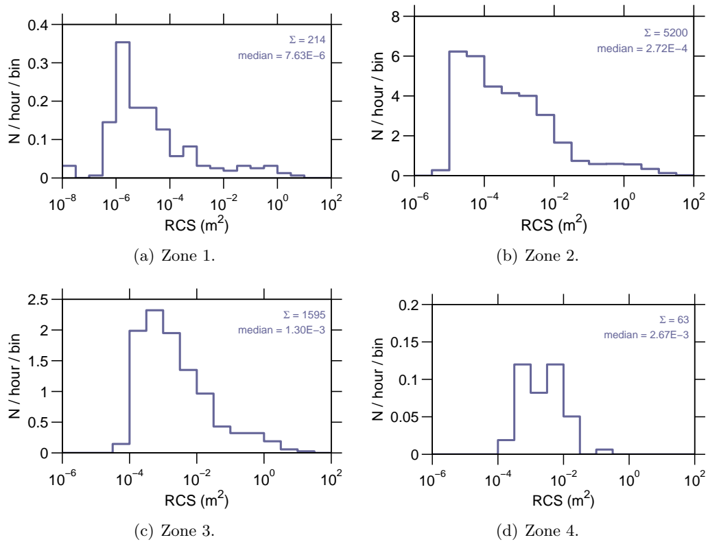
Figure 9: Event rate v radar cross section , 17 Sep–23 Sep 2007.
