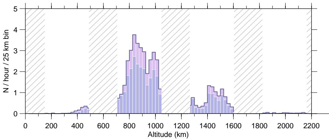
Figure 6: Event rate v altitude , 17 Sep–23 Sep 2007.
