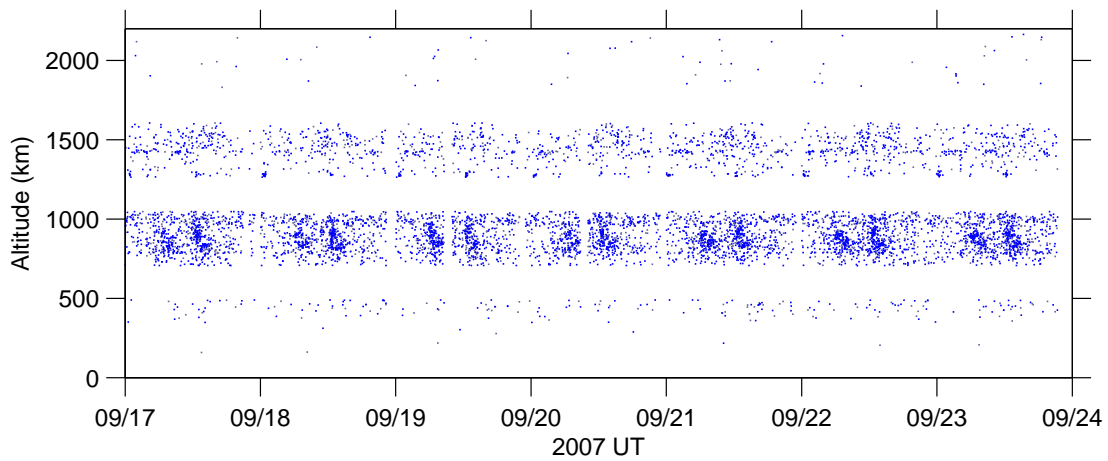
Figure 5: Altitude v time , 17 Sep–23 Sep 2007.
