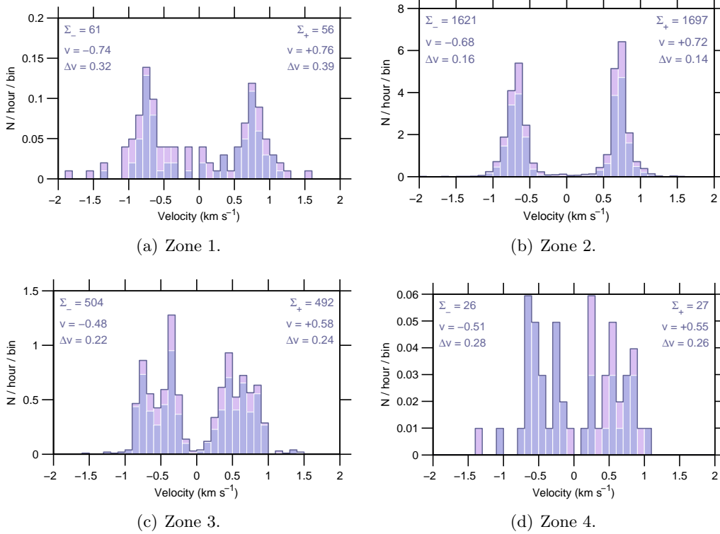
Figure 8: Event rate v Doppler-velocity , 10 Sep–16 Sep 2007.
