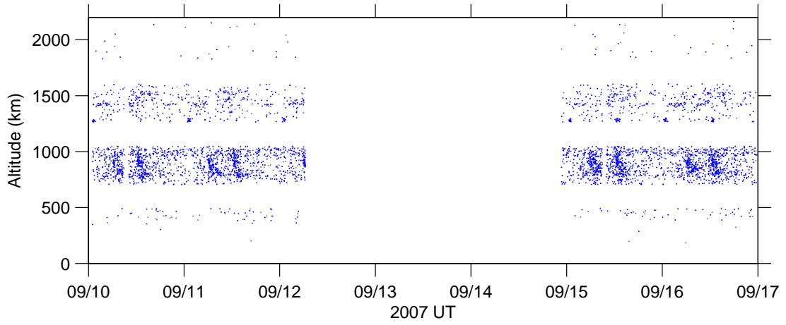
Figure 5: Altitude v time , 10 Sep–16 Sep 2007.
