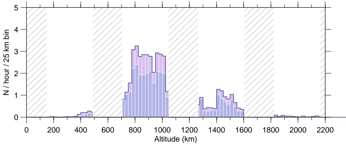
Figure 6: Event rate v altitude , 10 Sep–16 Sep 2007.
