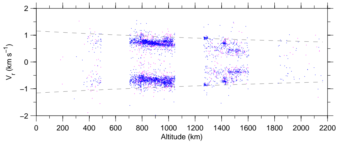
Figure 7: Doppler-velocity v altitude , 10 Sep–16 Sep 2007.
