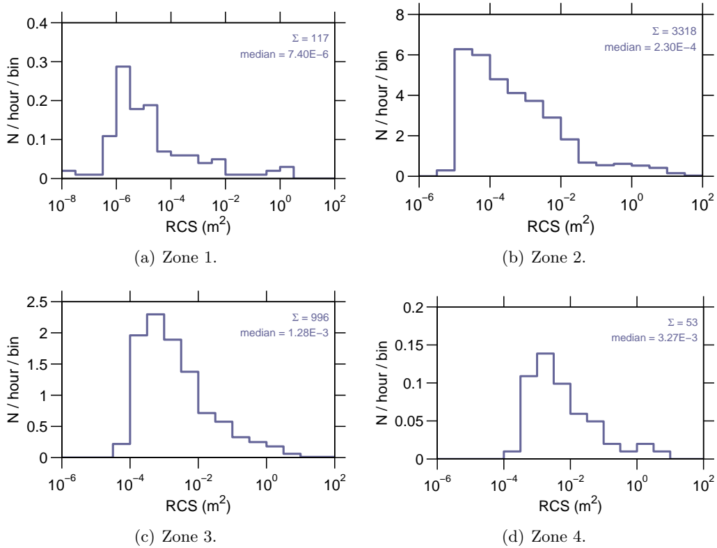
Figure 9: Event rate v radar cross section , 10 Sep–16 Sep 2007.
