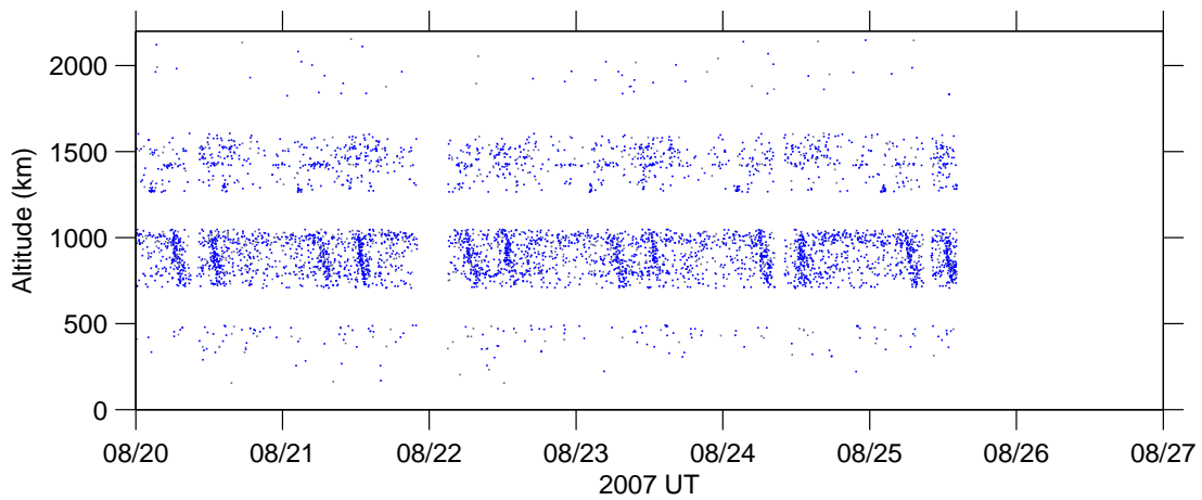
Figure 5: Altitude v time , 20 Aug–26 Aug 2007.
