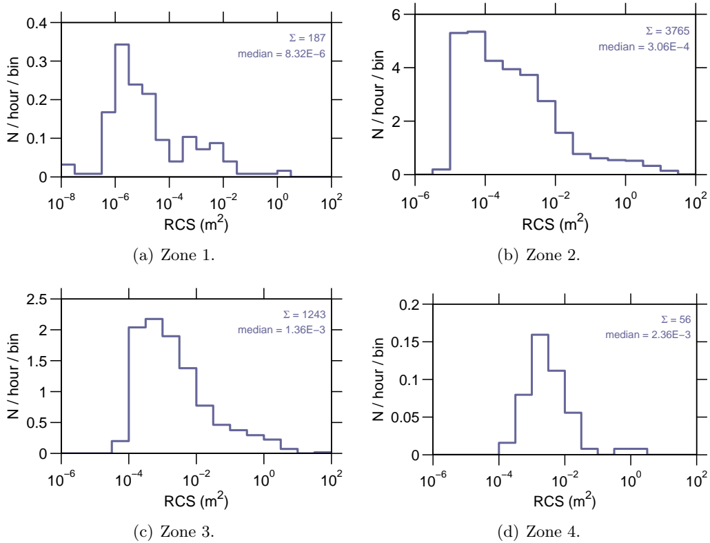
Figure 9: Event rate v radar cross section , 20 Aug–26 Aug 2007.
