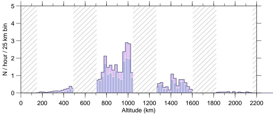
Figure 6: Event rate v altitude, 13 Aug–19 Aug 2007.
