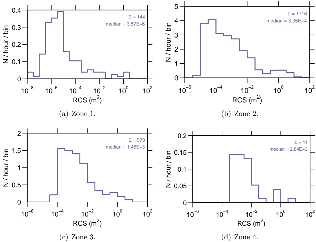
Figure 9: Event rate v radar cross section , 13 Aug–19 Aug 2007.
