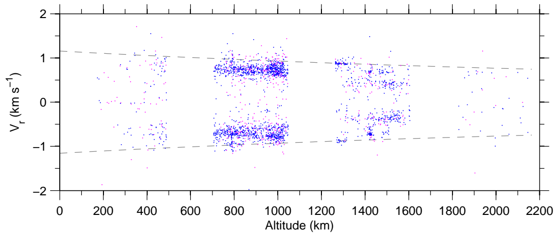
Figure 7: Doppler-velocity v altitude, 13 Aug–19 Aug 2007.
