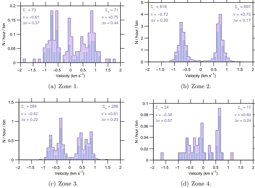
Figure 8: Event rate v Doppler-velocity , 13 Aug–19 Aug 2007.
