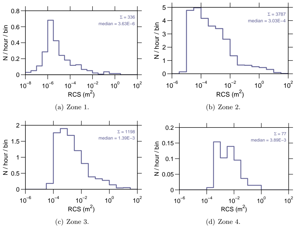
Figure 9: Event rate v radar cross section , 06 Aug–12 Aug 2007.
