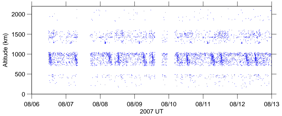
Figure 5: Altitude v time, 06 Aug–12 Aug 2007.
