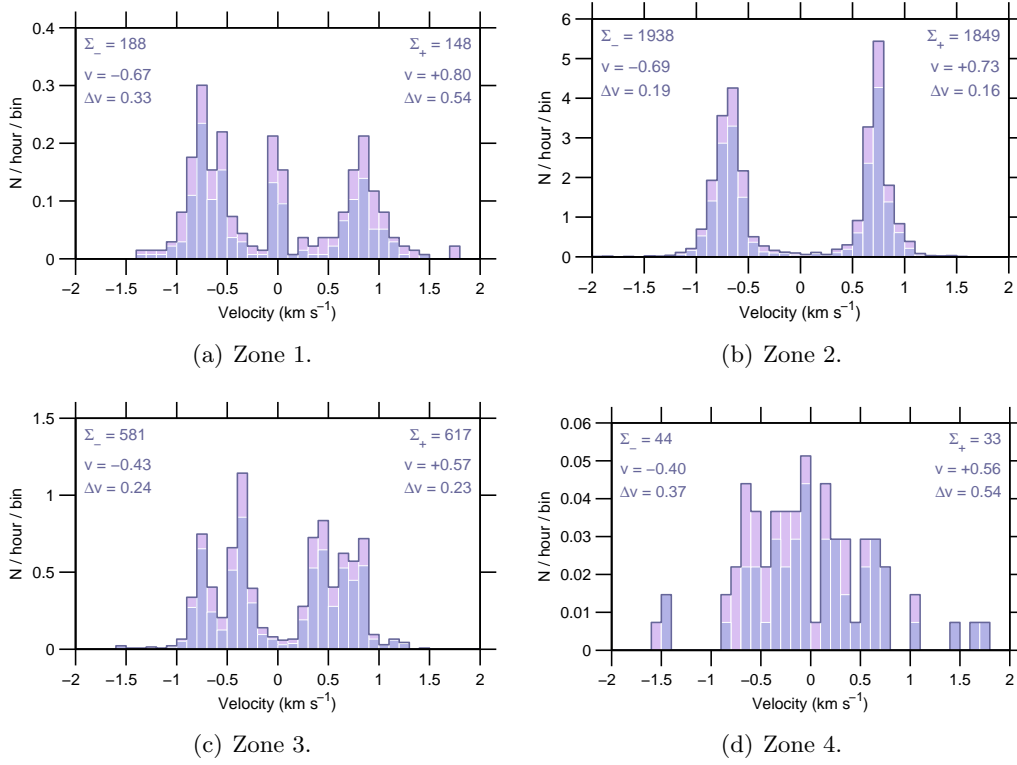
Figure 8: Event rate v Doppler-velocity , 06 Aug–12 Aug 2007.
