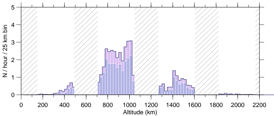
Figure 6: Event rate v altitude , 23 Jul–29 Jul 2007.
