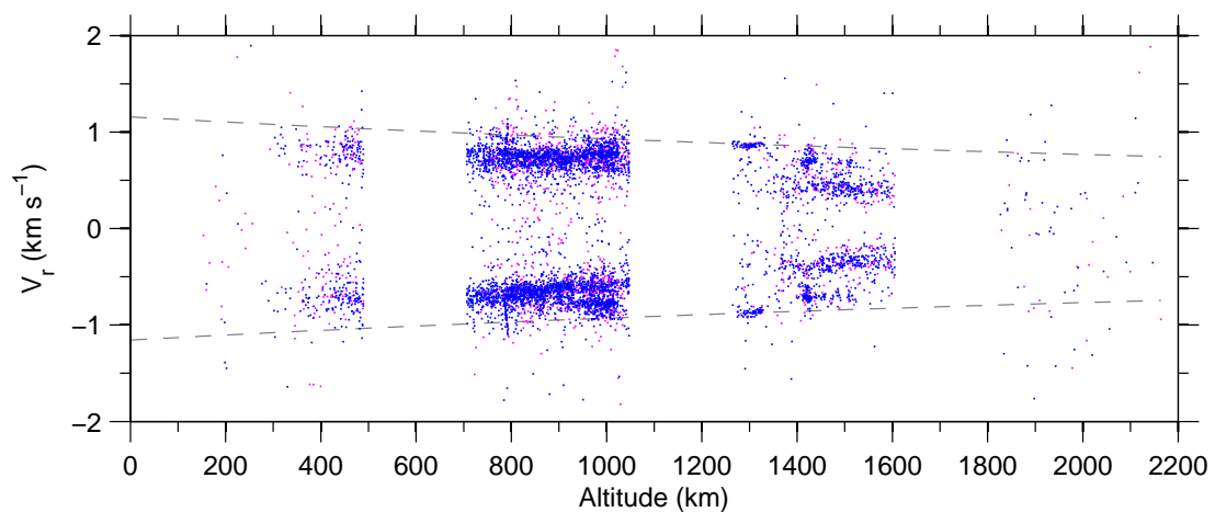
Figure 7: Doppler-velocity v altitude , 23 Jul–29 Jul 2007.
