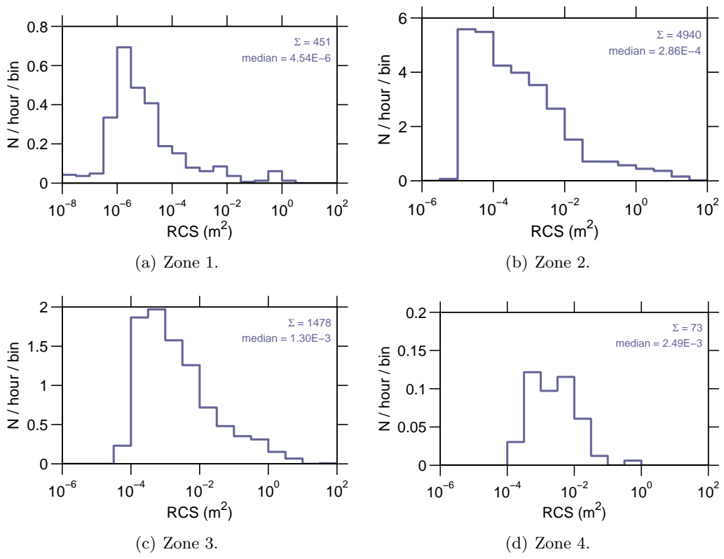
Figure 9: Event rate v radar cross section , 23 Jul–29 Jul 2007.
