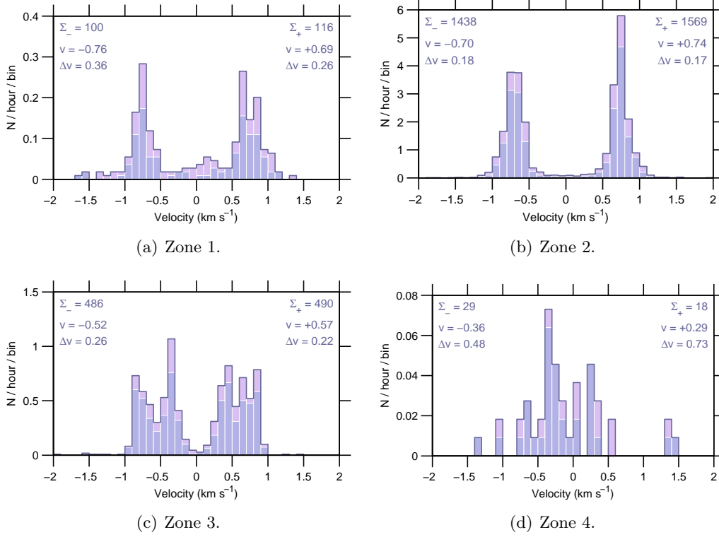
Figure 8: Event rate v Doppler-velocity , 02 Jul–08 Jul 2007.
