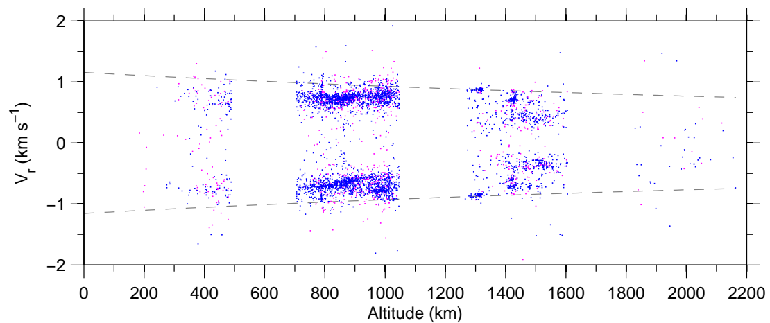
Figure 7: Doppler-velocity v altitude , 02 Jul–08 Jul 2007.
