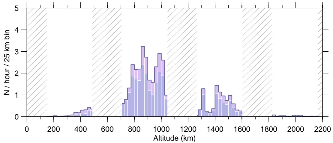
Figure 6: Event rate v altitude , 02 Jul–08 Jul 2007.
