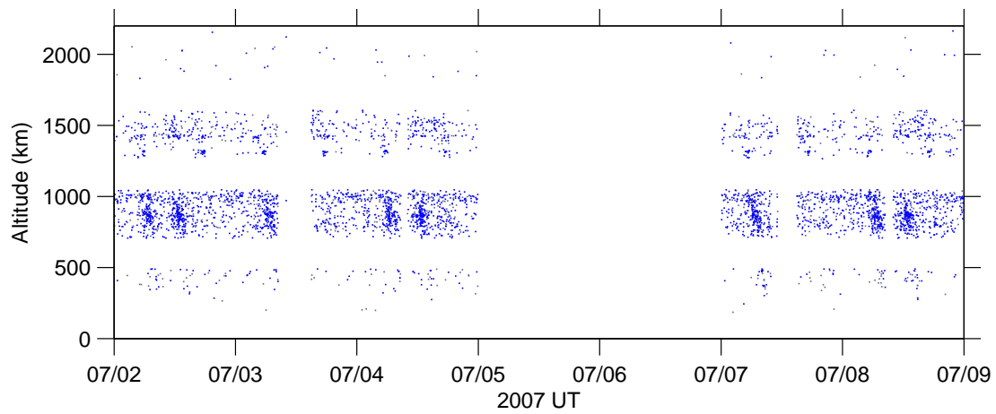
Figure 5: Altitude v time , 02 Jul–08 Jul 2007.
