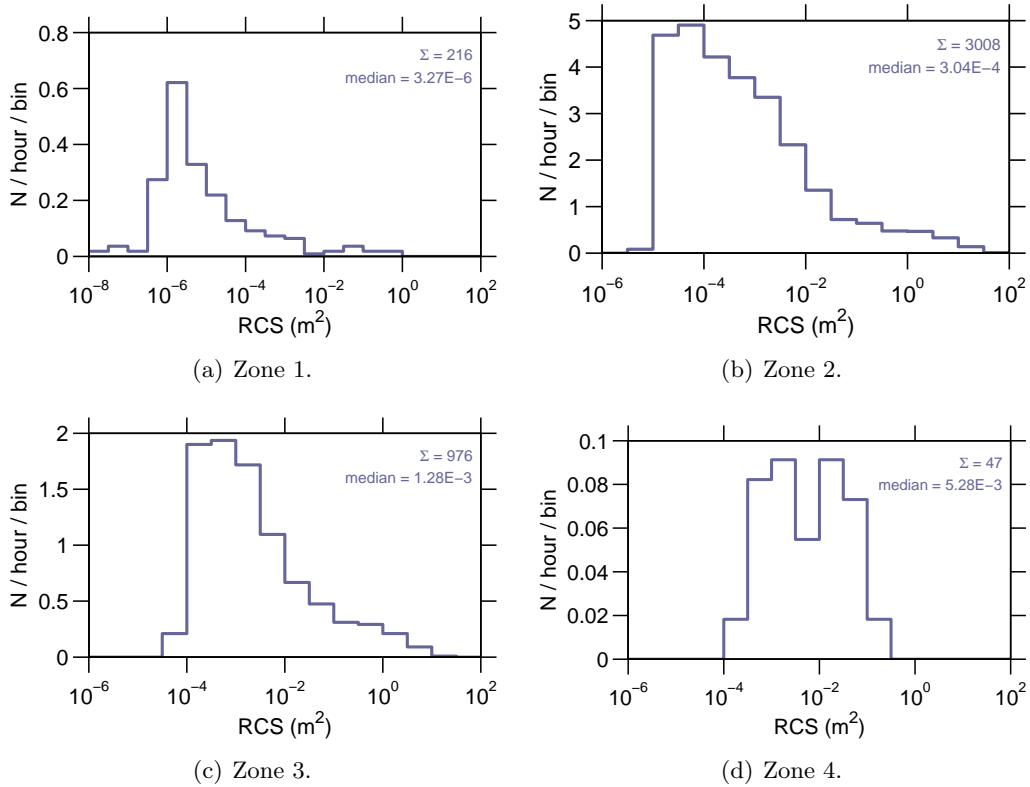
Figure 9: Event rate v radar cross section , 02 Jul–08 Jul 2007.
