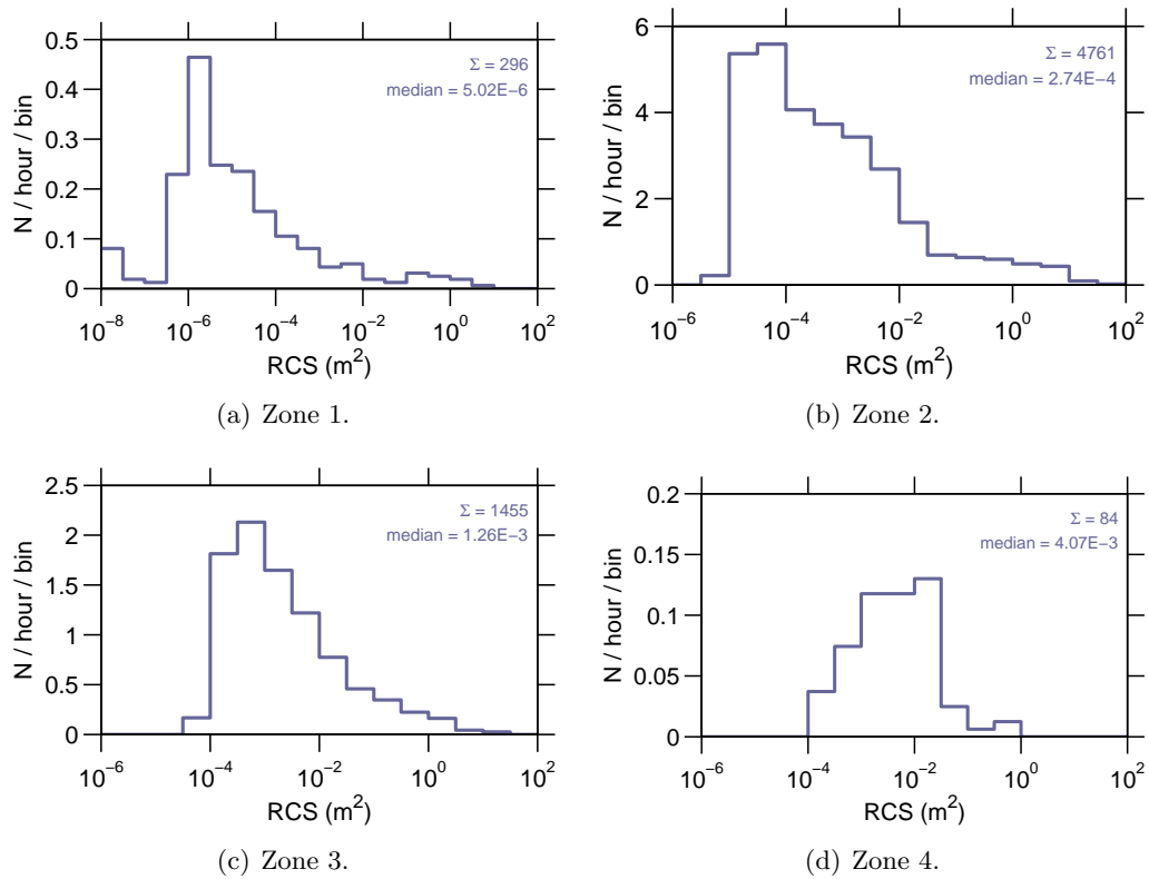
Figure 9: Event rate v radar cross section , 25 Jun–01 Jul 2007.
