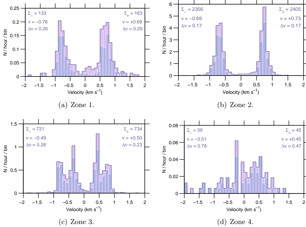
Figure 8: Event rate v Doppler-velocity , 25 Jun–01 Jul 2007.
