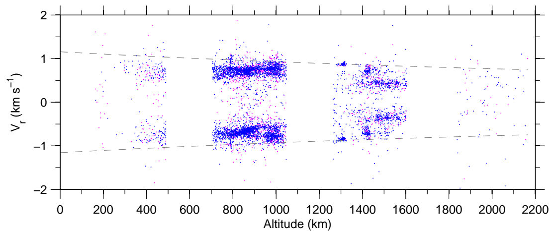
Figure 7: Doppler-velocity v altitude , 25 Jun–01 Jul 2007.
