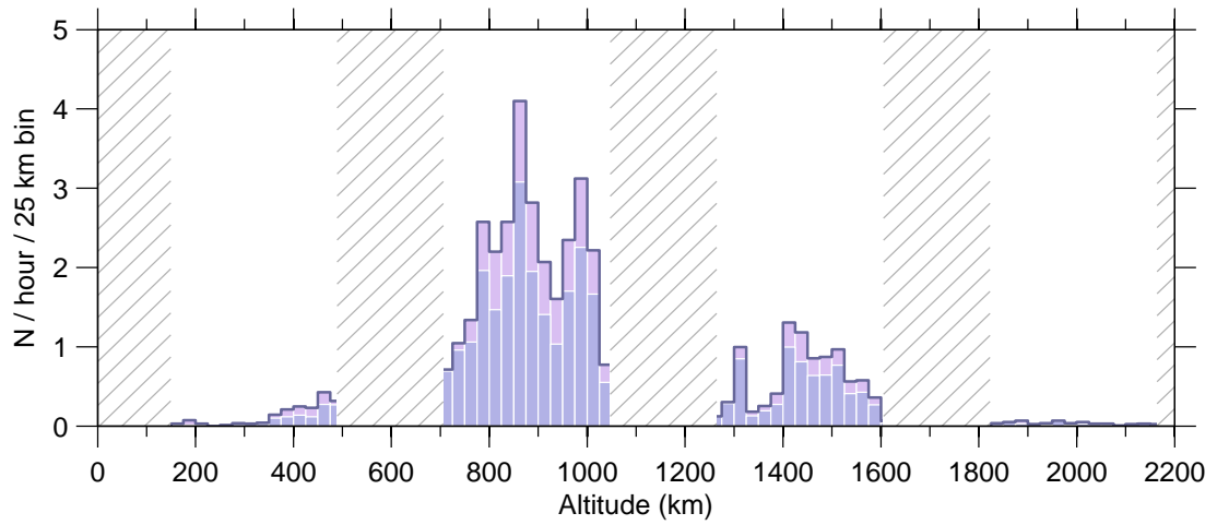
Figure 6: Event rate v altitude , 25 Jun–01 Jul 2007.
