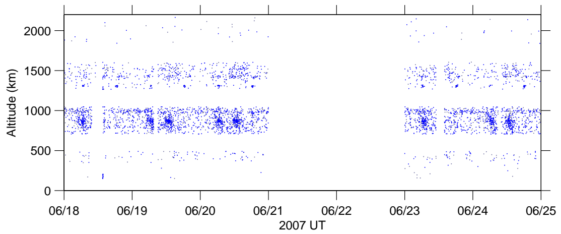
Figure 5: Altitude v time , 18 Jun–24 Jun 2007.
