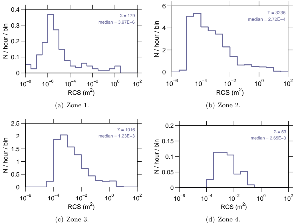
Figure 9: Event rate v radar cross section , 18 Jun–24 Jun 2007.
