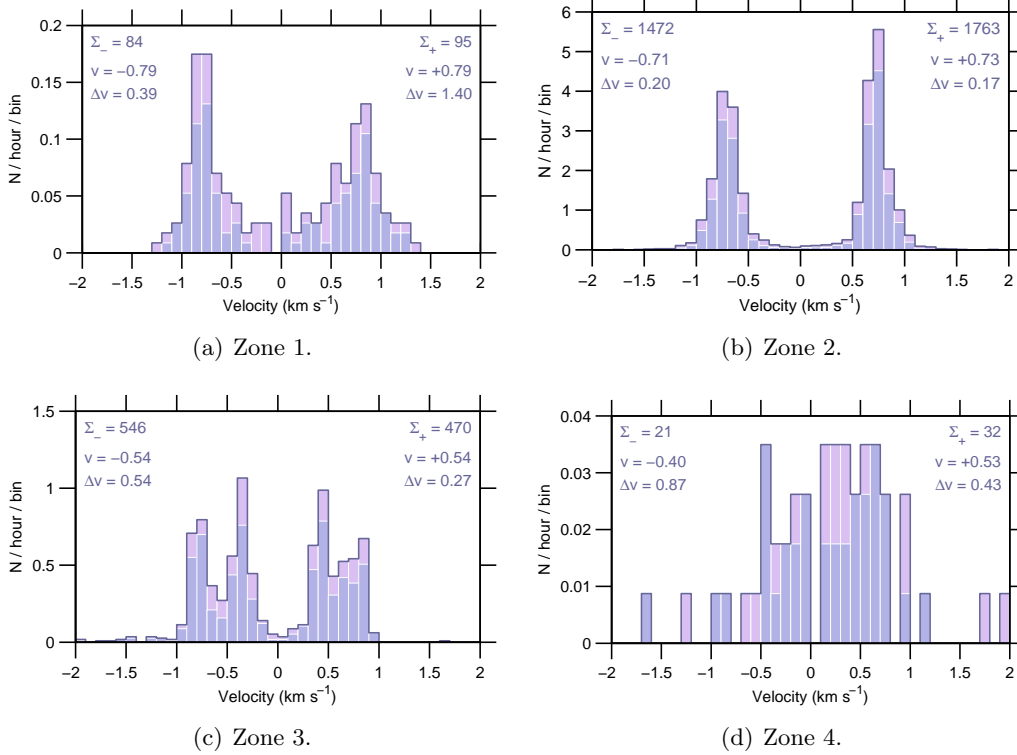
Figure 8: Event rate v Doppler-velocity , 18 Jun–24 Jun 2007.
