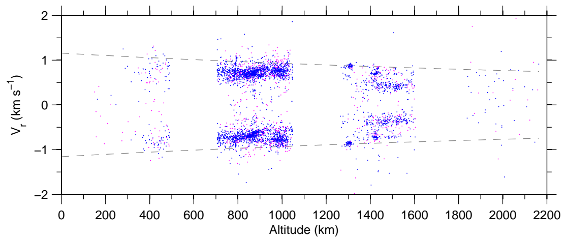
Figure 7: Doppler-velocity v altitude , 18 Jun–24 Jun 2007.
