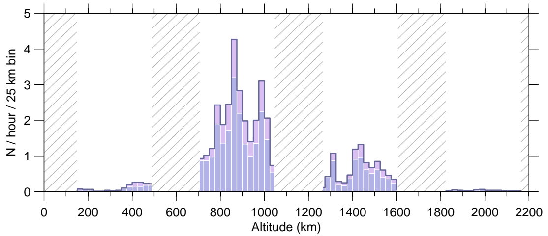
Figure 6: Event rate v altitude , 18 Jun–24 Jun 2007.
