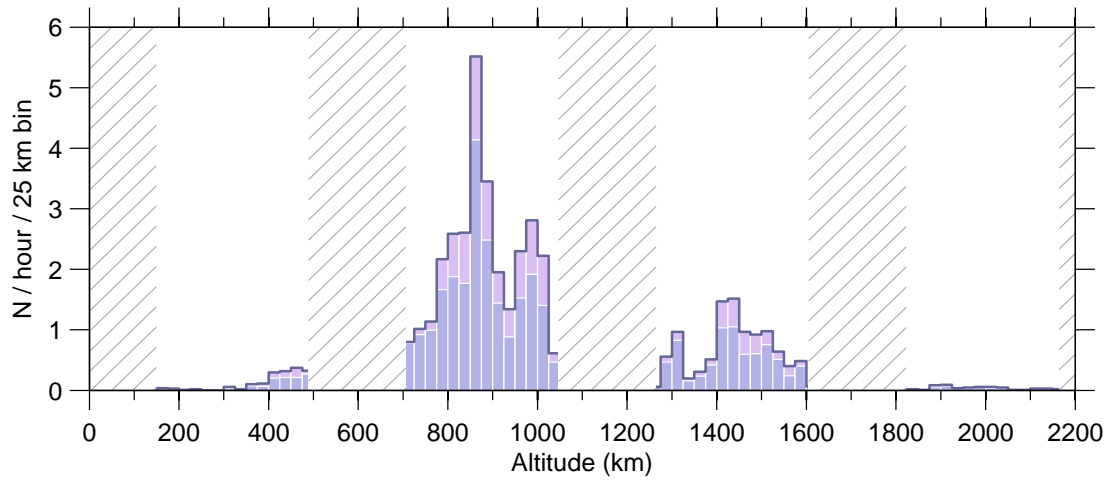
Figure 6: Event rate v altitude , 11 Jun–17 Jun 2007.
