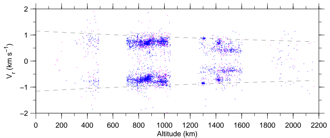
Figure 7: Doppler-velocity v altitude , 11 Jun–17 Jun 2007.
