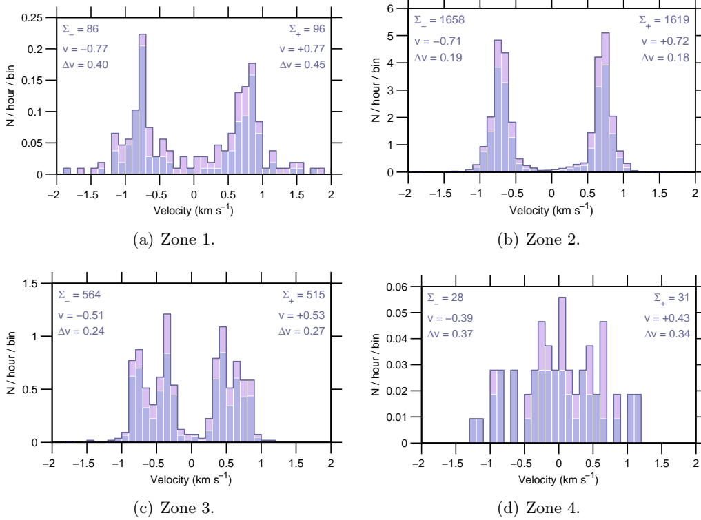
Figure 8: Event rate v Doppler-velocity , 11 Jun–17 Jun 2007.
