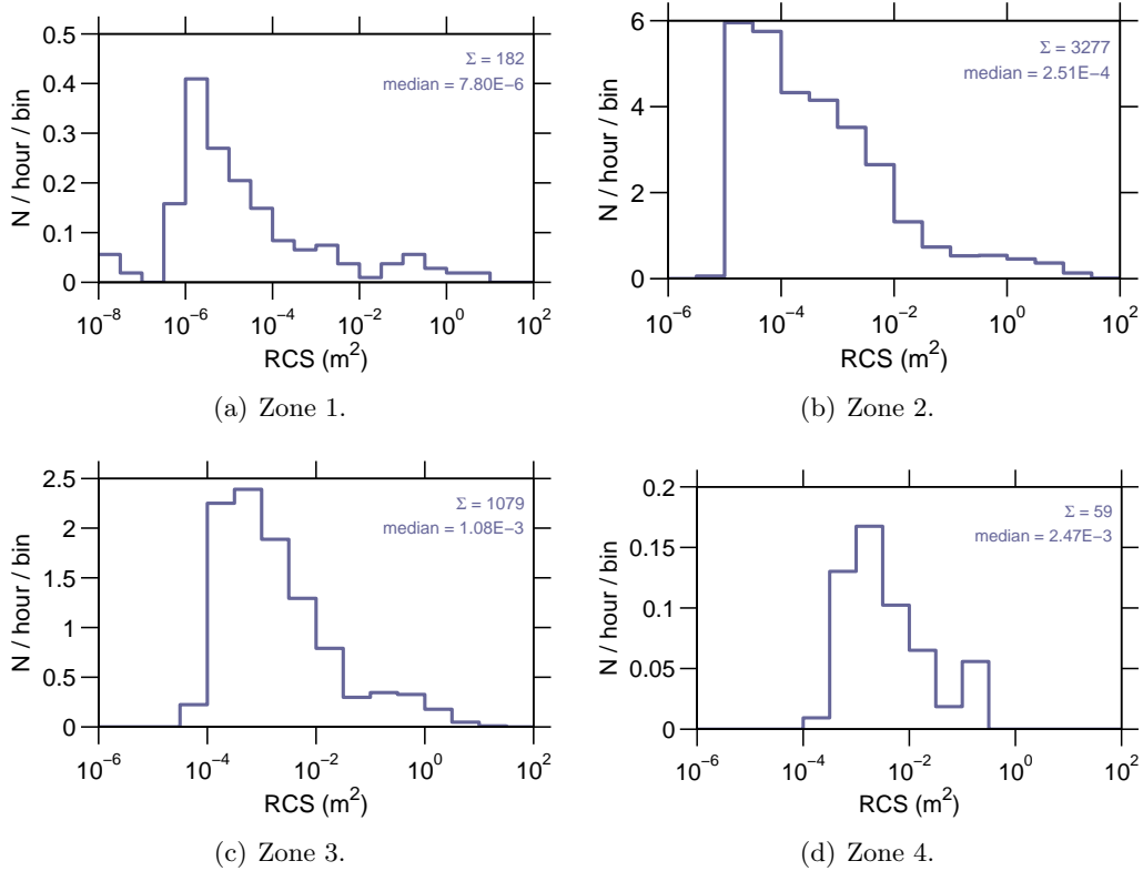
Figure 9: Event rate v radar cross section , 11 Jun–17 Jun 2007.
