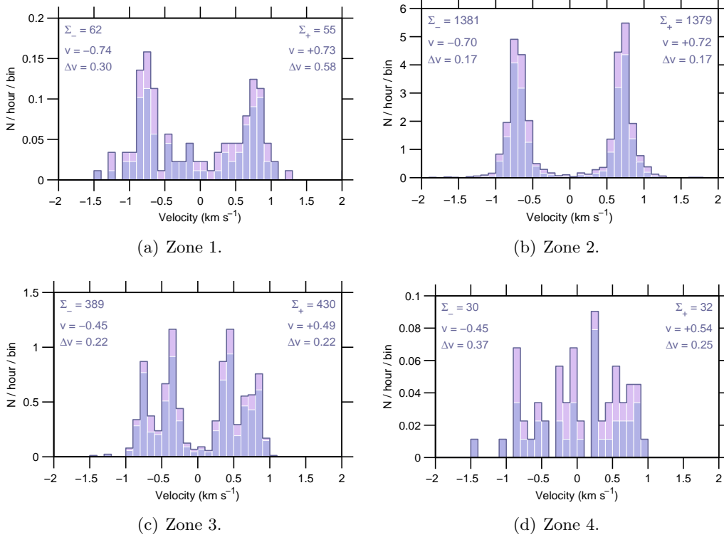
Figure 8: Event rate v Doppler-velocity, 04 Jun–10 Jun 2007.
