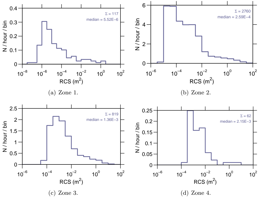
Figure 9: Event rate v radar cross section, 04 Jun–10 Jun 2007.
