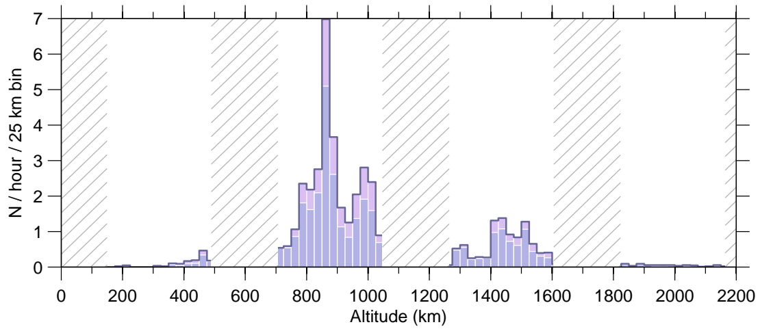
Figure 6: Event rate v altitude , 04 Jun–10 Jun 2007.
