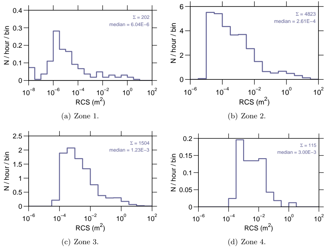
Figure 9: Event rate v radar cross section , 28 May–03 Jun 2007.
