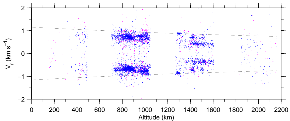
Figure 7: Doppler-velocity v altitude , 28 May–03 Jun 2007.
