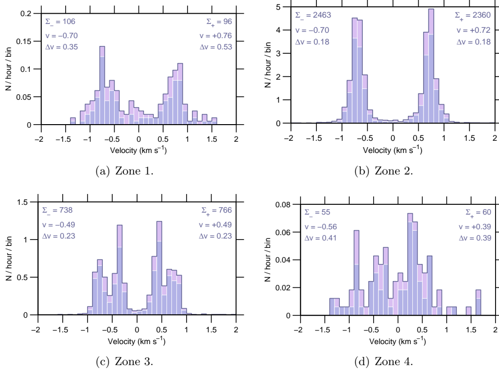
Figure 8: Event rate v Doppler-velocity , 28 May–03 Jun 2007.
