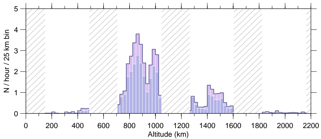
Figure 6: Event rate v altitude , 21 May–27 May 2007.
