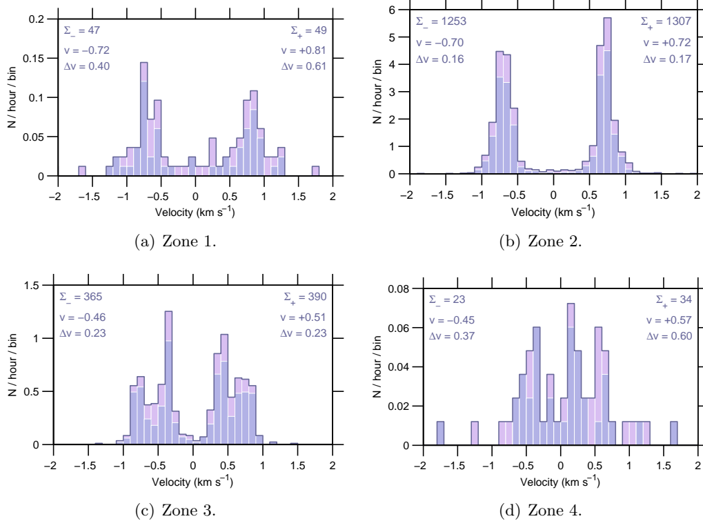
Figure 8: Event rate v Doppler-velocity , 21 May–27 May 2007.
