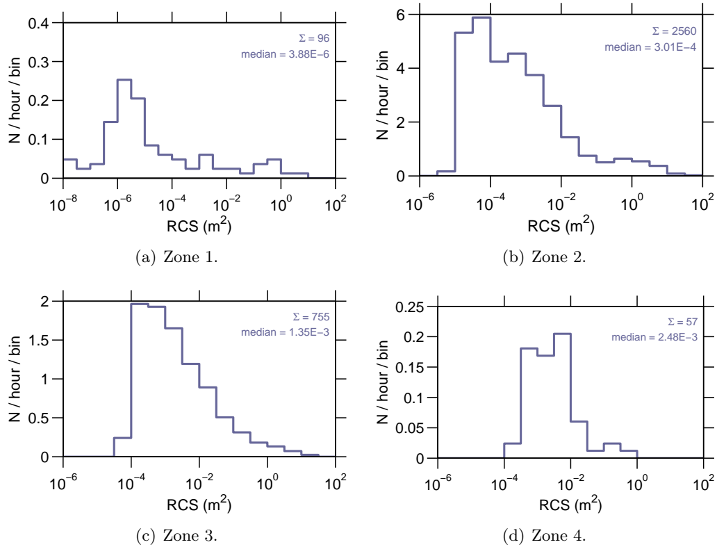
Figure 9: Event rate v radar cross section , 21 May–27 May 2007.
