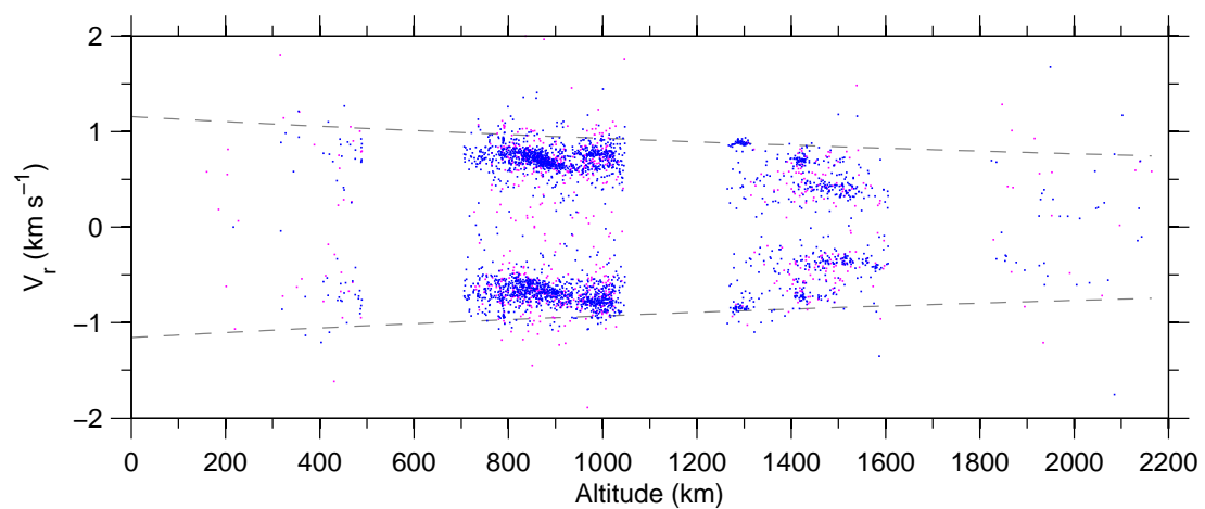
Figure 7: Doppler-velocity v altitude , 21 May–27 May 2007.
