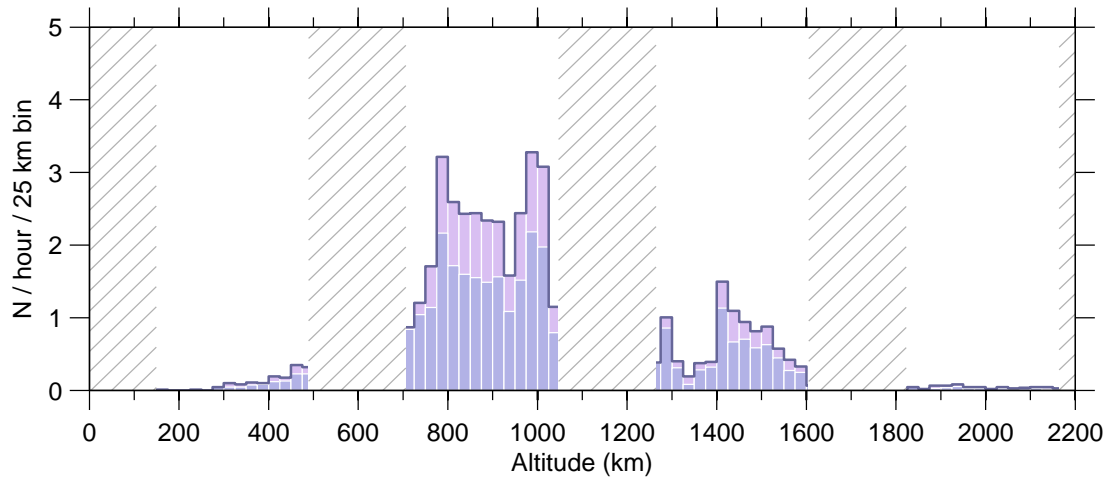
Figure 6: Event rate v altitude , 07 May–13 May 2007.
