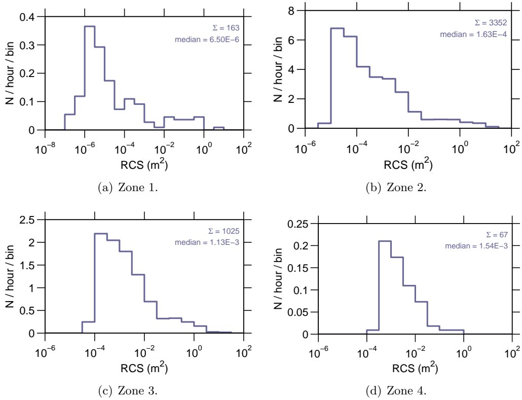
Figure 9: Event rate v radar cross section , 07 May–13 May 2007.
