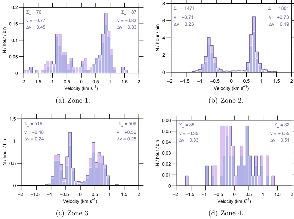
Figure 8: Event rate v Doppler-velocity , 07 May–13 May 2007.
