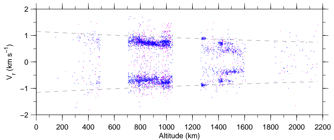
Figure 7: Doppler-velocity v altitude , 07 May–13 May 2007.
