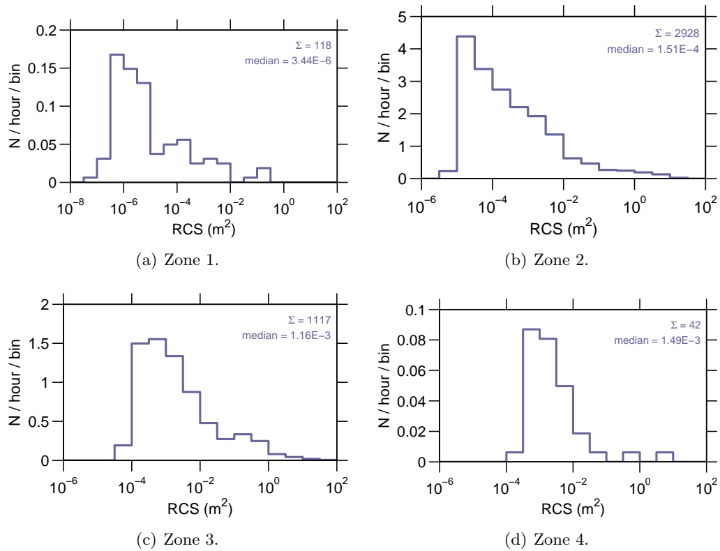
Figure 9: Event rate v radar cross section , 30 Apr–06 May 2007.
