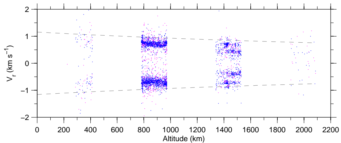
Figure 7: Doppler-velocity v altitude , 30 Apr–06 May 2007.
