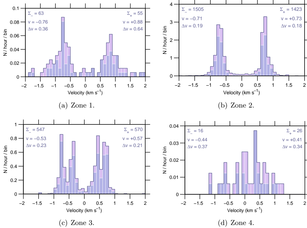
Figure 8: Event rate v Doppler-velocity , 30 Apr–06 May 2007.
