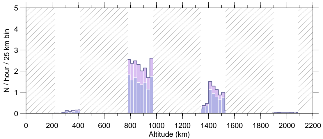
Figure 6: Event rate v altitude , 30 Apr–06 May 2007.
