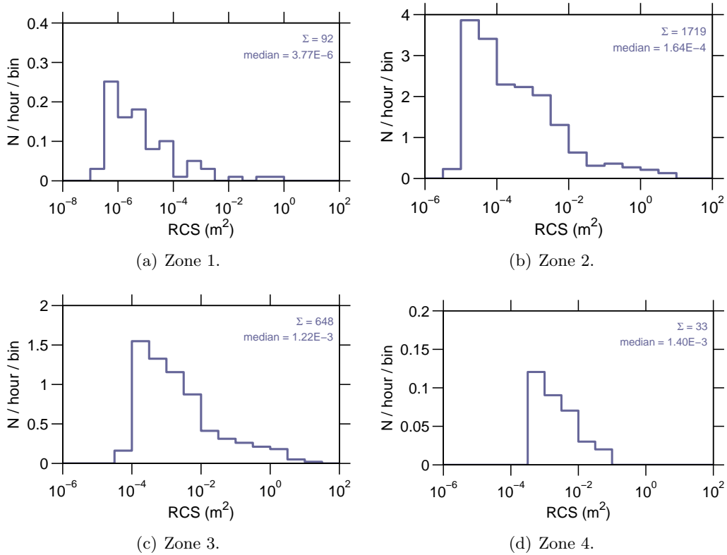
Figure 9: Event rate v radar cross section , 16 Apr–22 Apr 2007.
