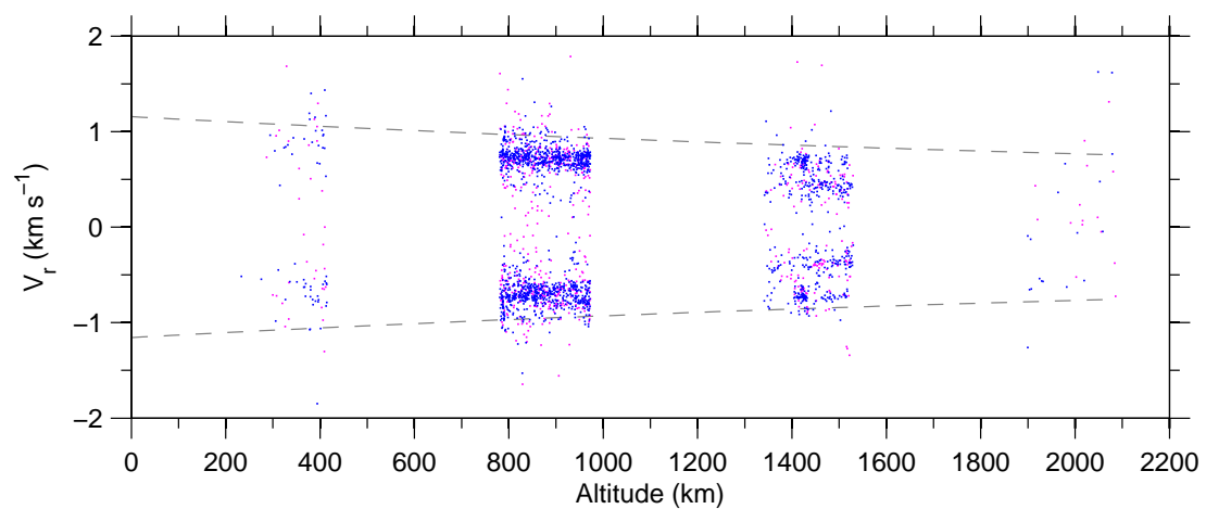
Figure 7: Doppler-velocity v altitude , 16 Apr–22 Apr 2007.
