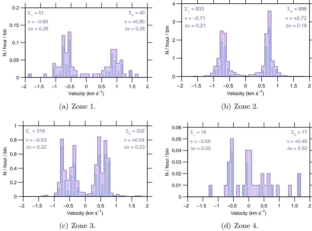
Figure 8: Event rate v Doppler-velocity , 16 Apr–22 Apr 2007.
