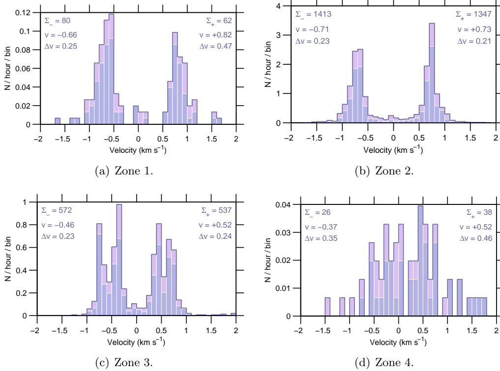
Figure 8: Event rate v Doppler-velocity , 09 Apr–15 Apr 2007.
