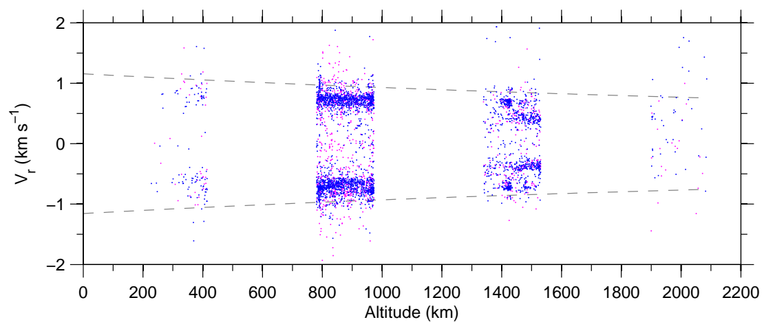
Figure 7: Doppler-velocity v altitude , 09 Apr–15 Apr 2007.
