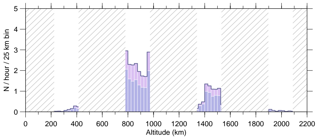
Figure 6: Event rate v altitude , 09 Apr–15 Apr 2007.
