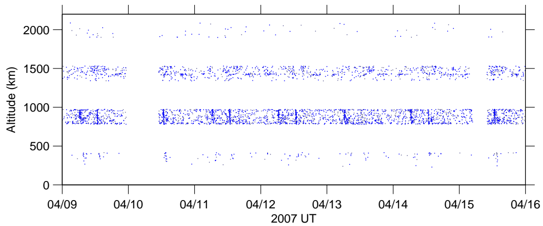
Figure 5: Altitude v time , 09 Apr–15 Apr 2007.
