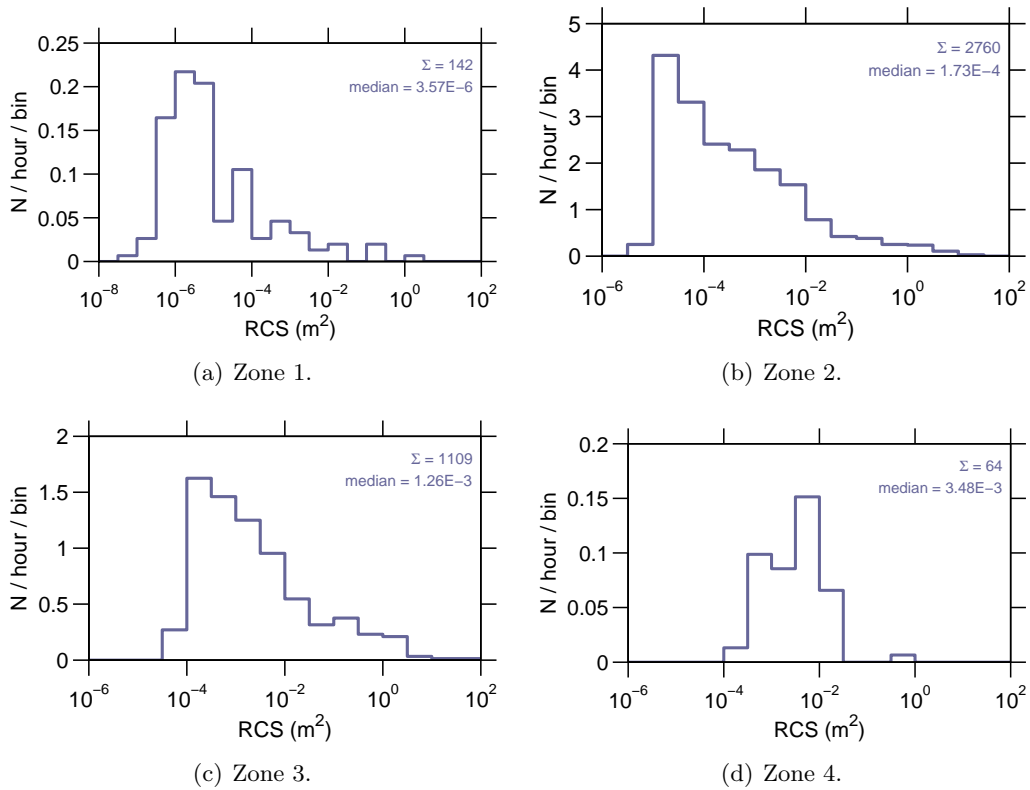
Figure 9: Event rate v radar cross section , 09 Apr–15 Apr 2007.
