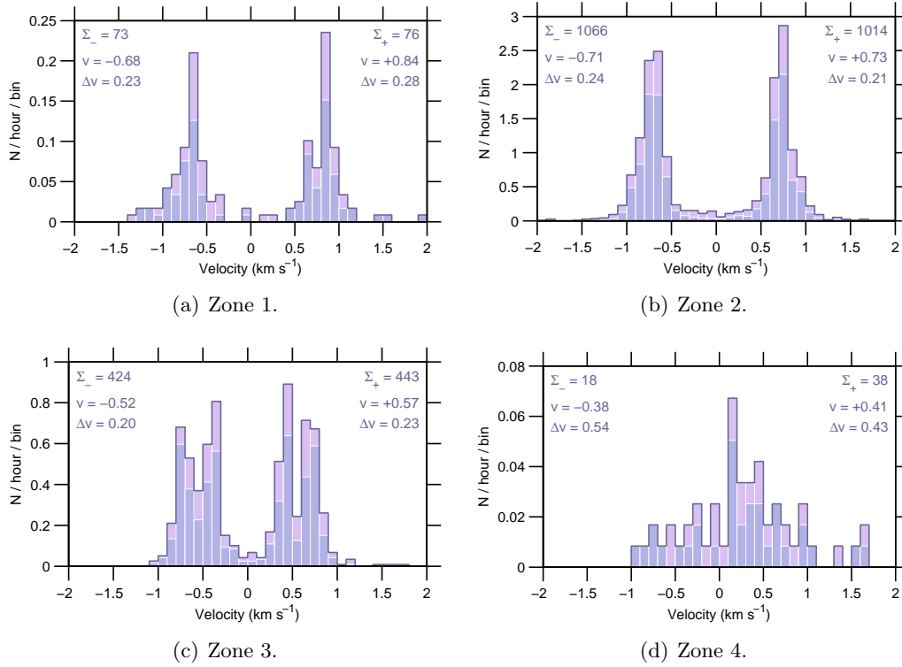
Figure 8: Event rate v Doppler-velocity, 02 Apr–08 Apr 2007.
