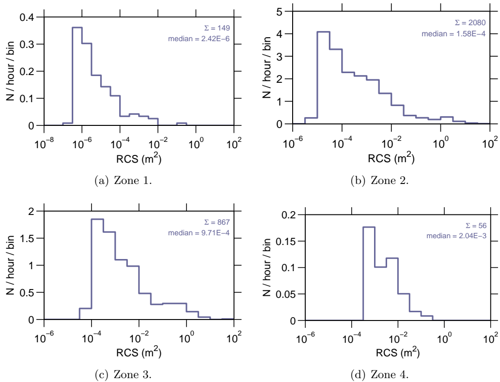
Figure 9: Event rate v radar cross section, 02 Apr–08 Apr 2007.
