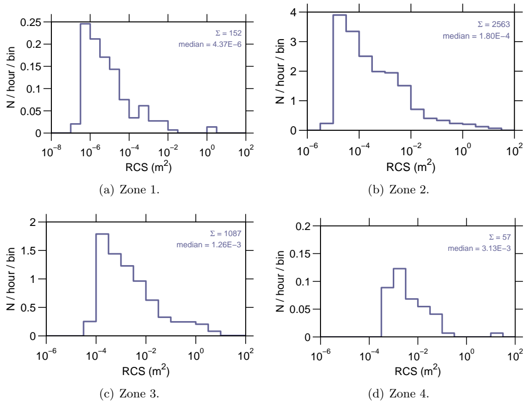
Figure 9: Event rate v radar cross section , 26 Mar–01 Apr 2007.
