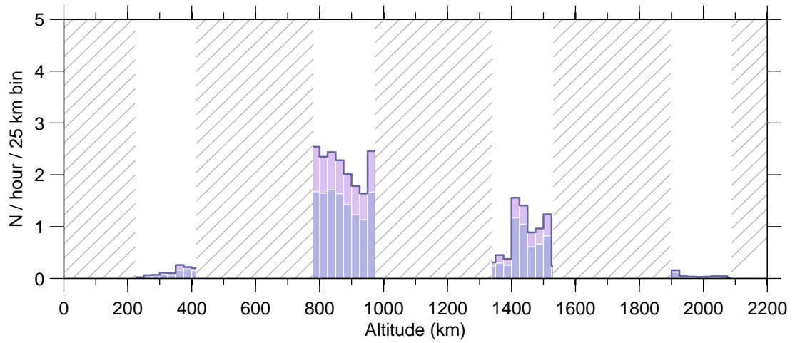
Figure 6: Event rate v altitude , 26 Mar–01 Apr 2007.
