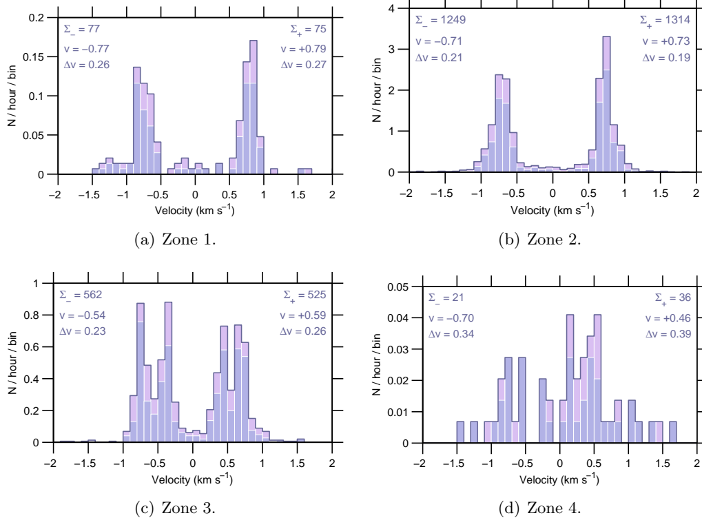
Figure 8: Event rate v Doppler-velocity , 26 Mar–01 Apr 2007.
