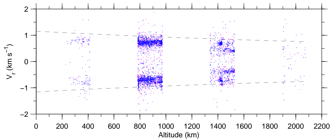
Figure 7: Doppler-velocity v altitude , 26 Mar–01 Apr 2007.
