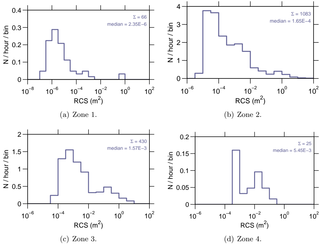
Figure 9: Event rate v radar cross section , 19 Mar–25 Mar 2007.
