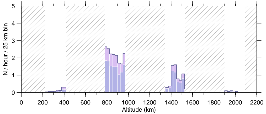
Figure 6: Event rate v altitude , 19 Mar–25 Mar 2007.
