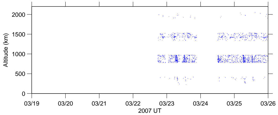
Figure 5: Altitude v time , 19 Mar–25 Mar 2007.
