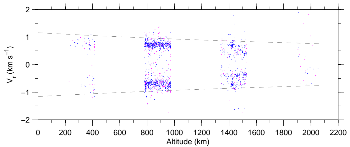
Figure 7: Doppler-velocity v altitude , 19 Mar–25 Mar 2007.
