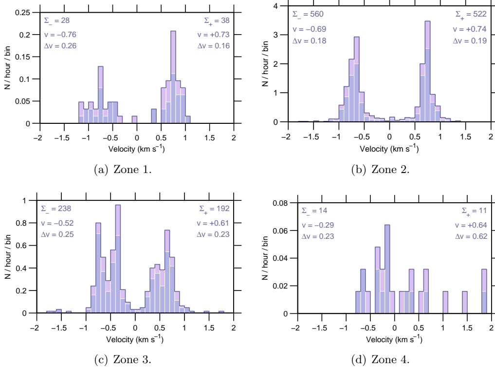
Figure 8: Event rate v Doppler-velocity , 19 Mar–25 Mar 2007.
