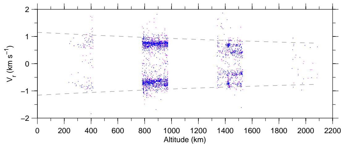
Figure 7: Doppler-velocity v altitude , 12 Mar–18 Mar 2007.
