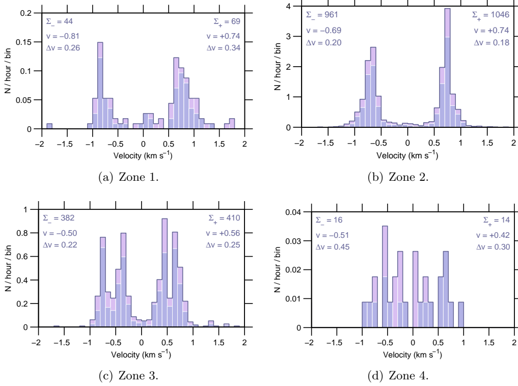
Figure 8: Event rate v Doppler-velocity , 12 Mar–18 Mar 2007.
