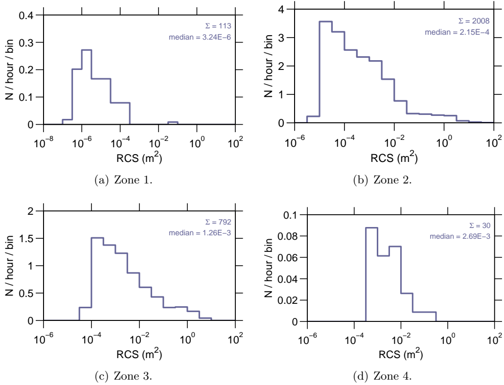
Figure 9: Event rate v radar cross section , 12 Mar–18 Mar 2007.
