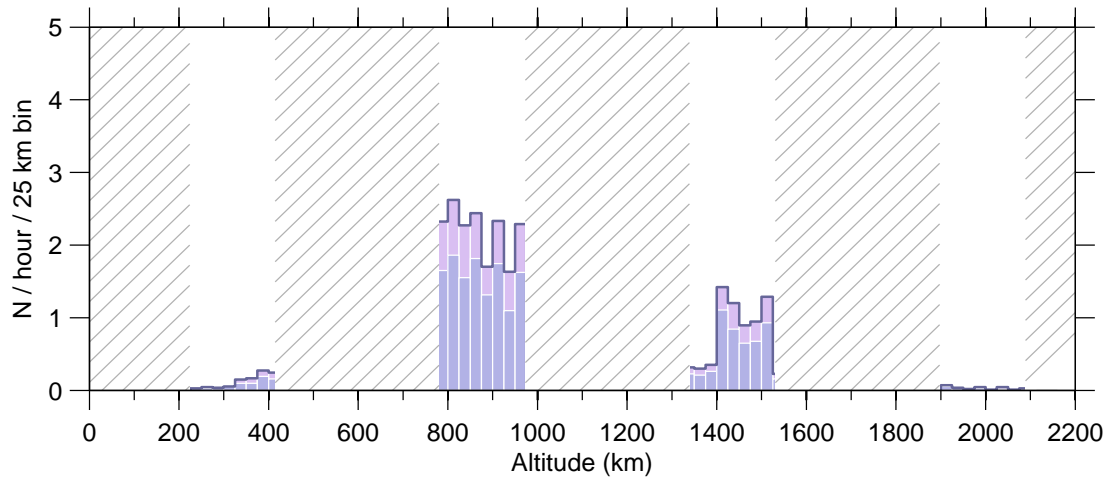
Figure 6: Event rate v altitude , 12 Mar–18 Mar 2007.
