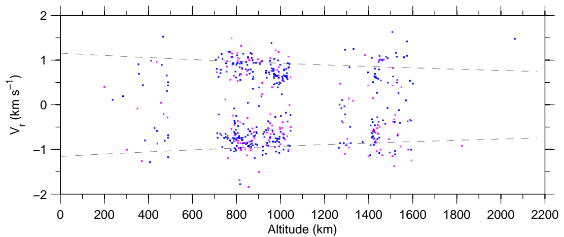
Figure 7: Doppler-velocity v altitude on 22-May-2008.
