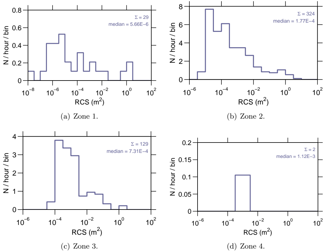
Figure 9: Event rate v RCS on 22-May-2008.
