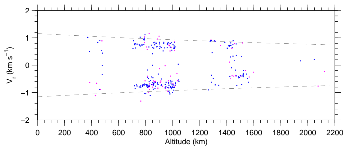
Figure 7: Doppler-velocity v altitude on 13-February-2008.
