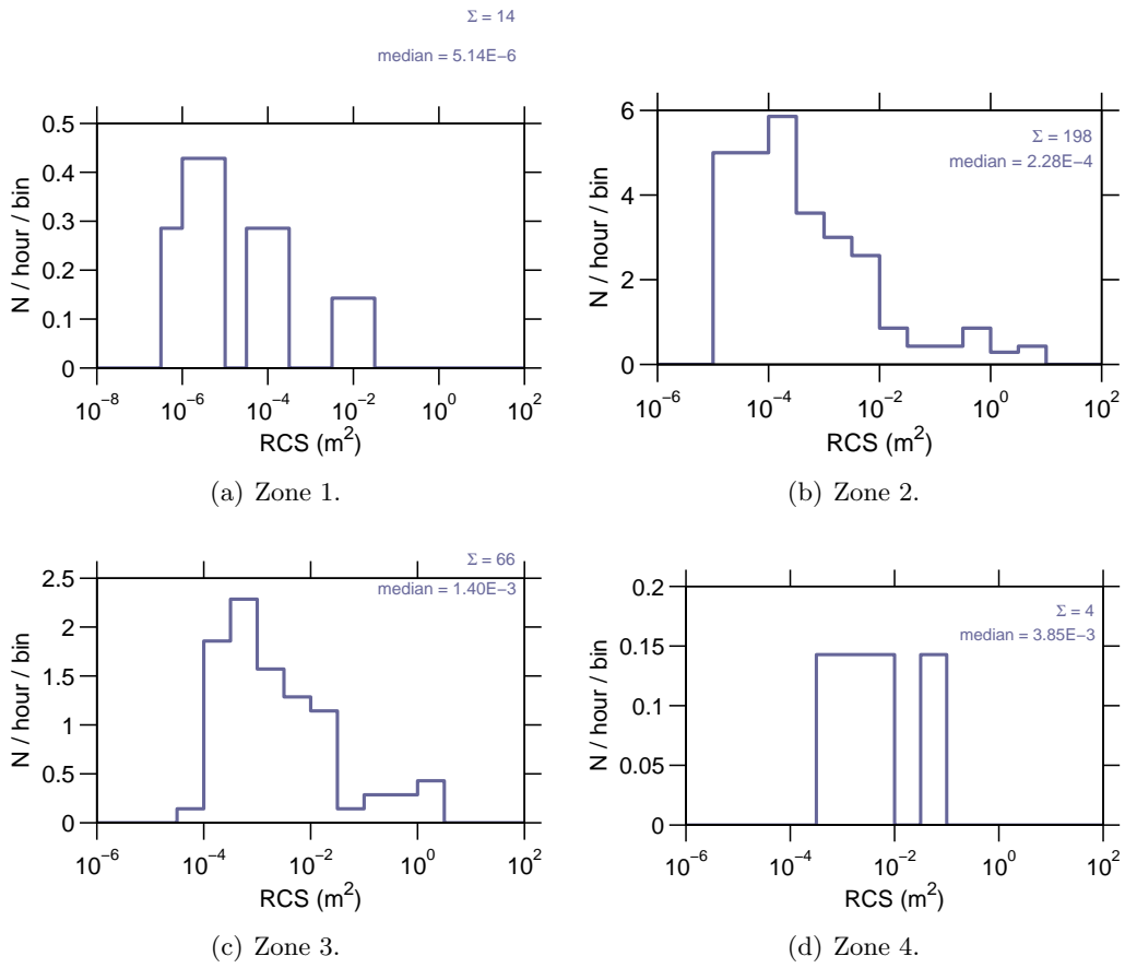
Figure 9: Event rate v RCS on 13-February-2008.
