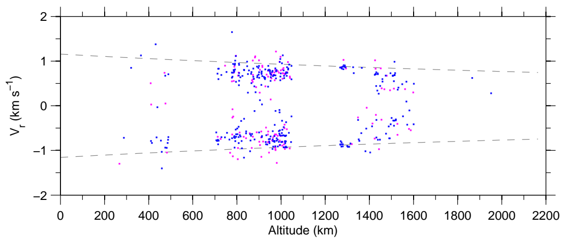
Figure 7: Doppler-velocity v altitude on 15-January-2008.
