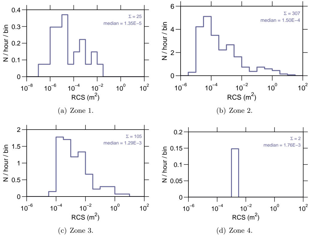
Figure 9: Event rate v RCS on 15-January-2008.
