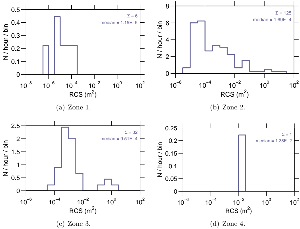
Figure 9: Event rate v RCS on 06-January-2008.
