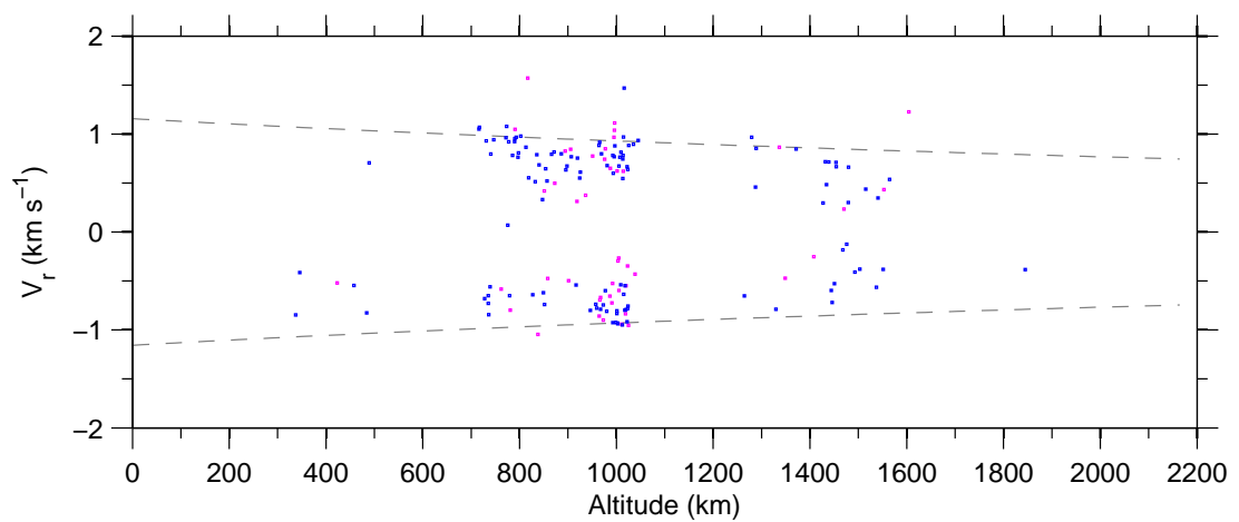
Figure 7: Doppler-velocity v altitude on 06-January-2008.
