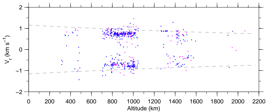
Figure 7: Doppler-velocity v altitude on 28-November-2007.
