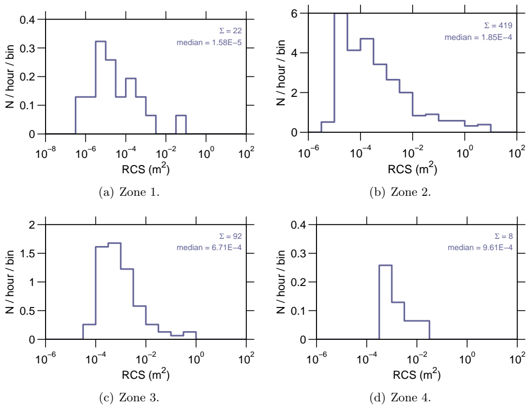
Figure 9: Event rate v RCS on 28-November-2007.
