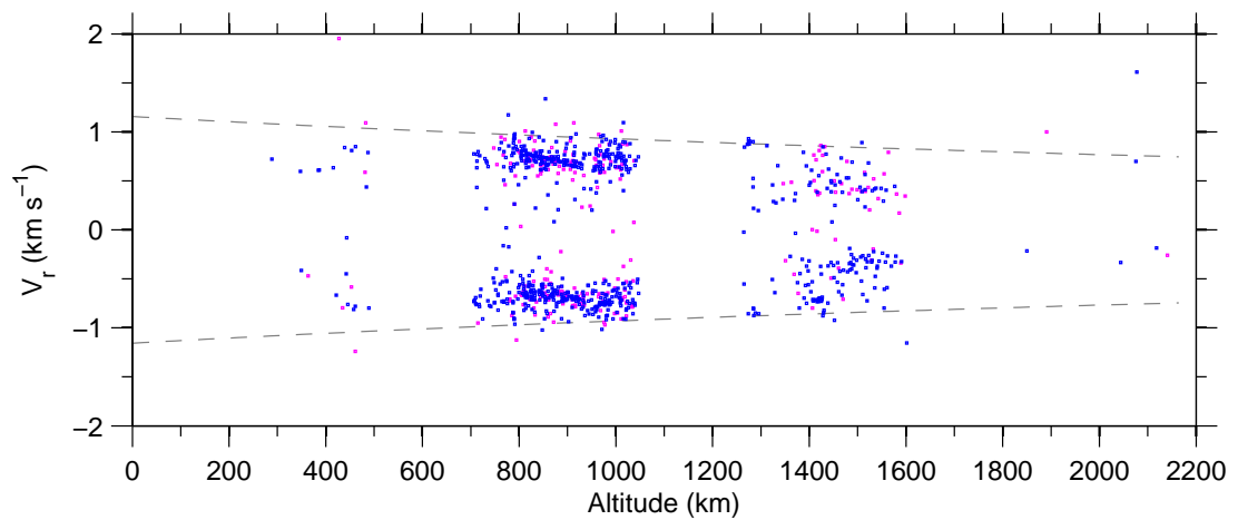
Figure 7: Doppler-velocity v altitude on 20-September-2007.
