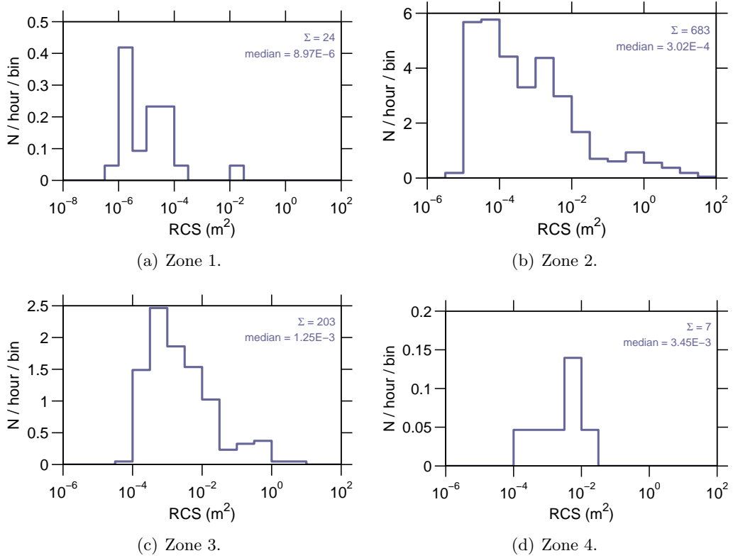
Figure 9: Event rate v RCS on 20-September-2007.
