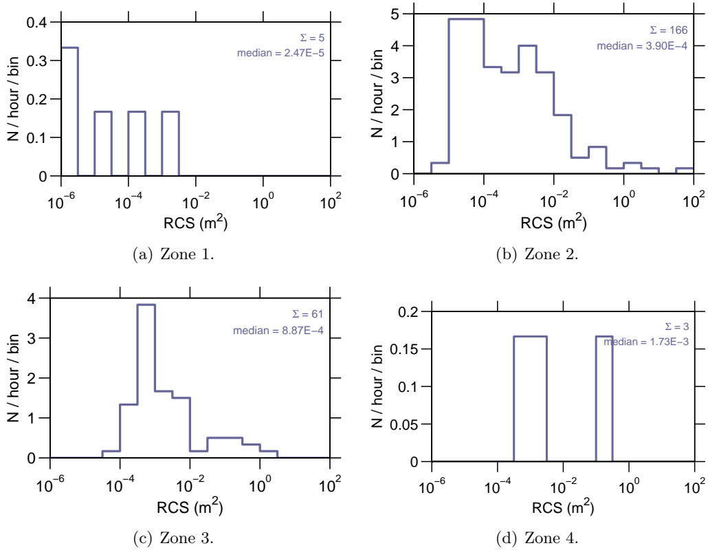
Figure 9: Event rate v RCS on 12-September-2007.
