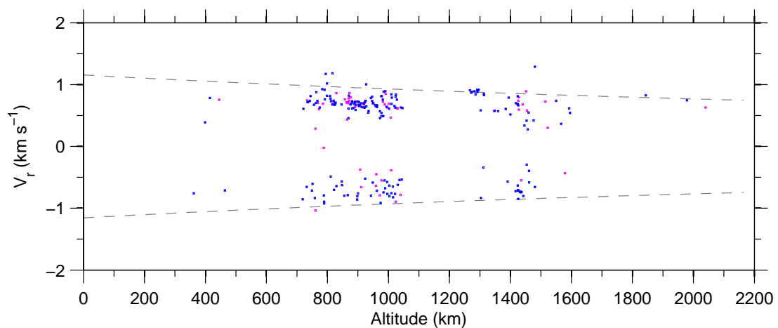
Figure 7: Doppler-velocity v altitude on 12-September-2007.
