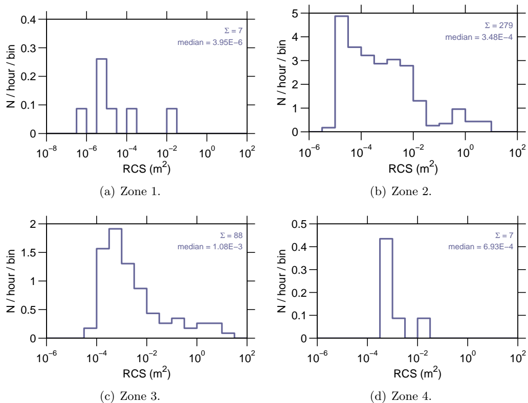
Figure 9: Event rate v RCS on 09-September-2007.
