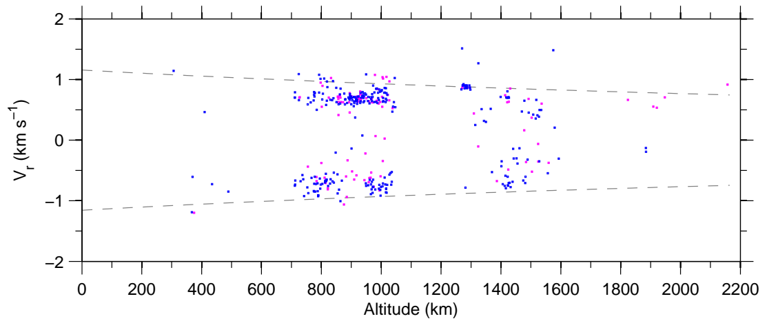
Figure 7: Doppler-velocity v altitude on 09-September-2007.
