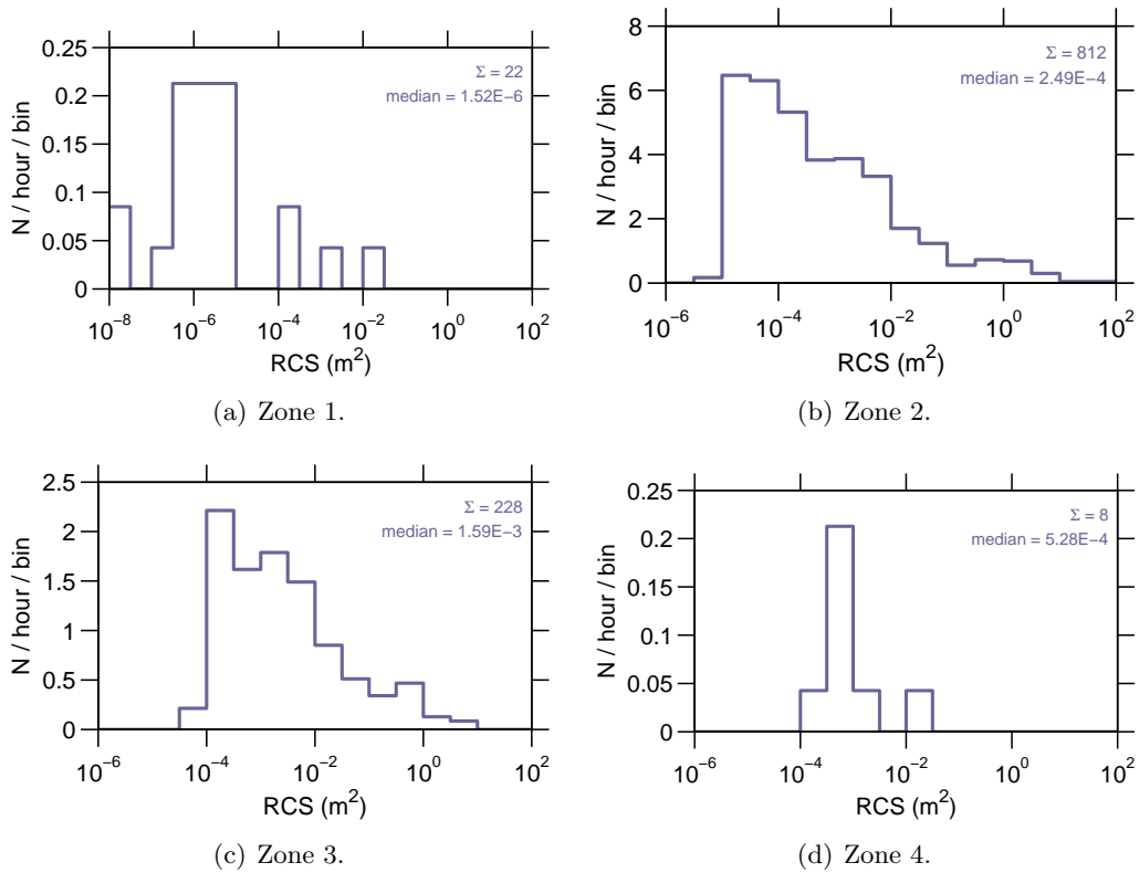
Figure 9: Event rate v RCS on 08-September-2007.
