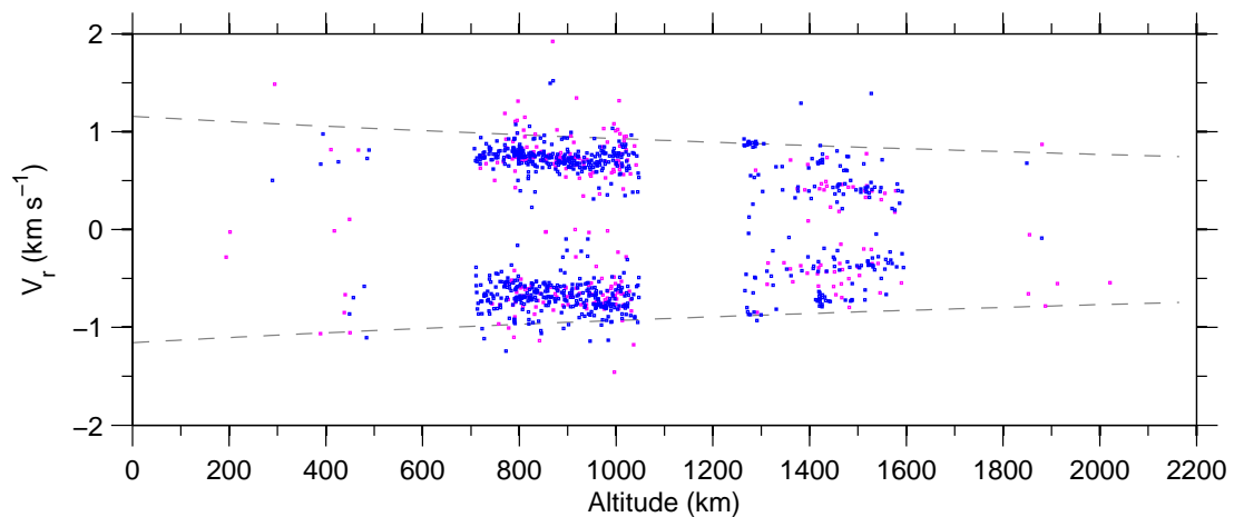
Figure 7: Doppler-velocity v altitude on 08-September-2007.
