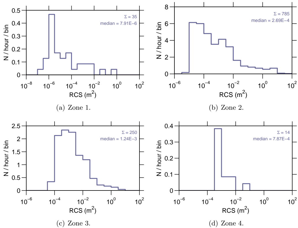
Figure 9: Event rate v RCS on 07-September-2007.
