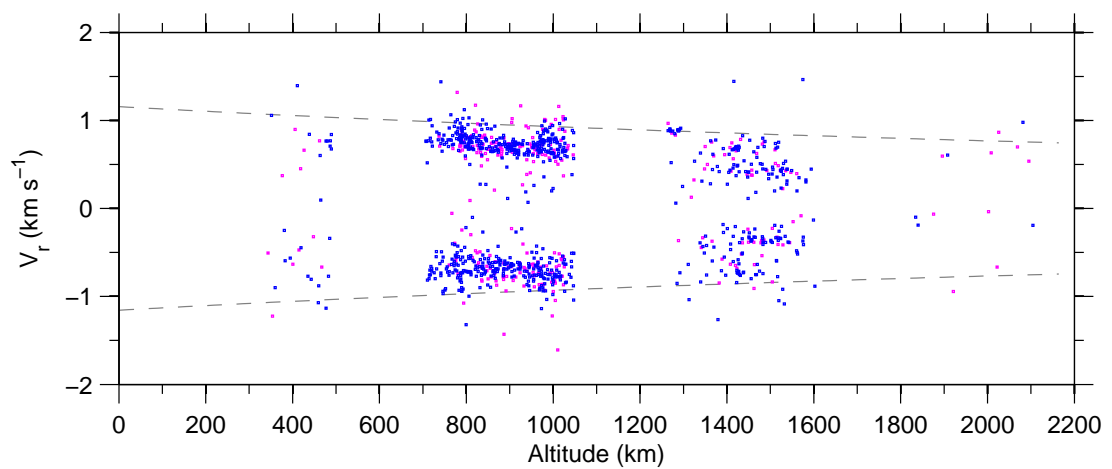
Figure 7: Doppler-velocity v altitude on 07-September-2007.
