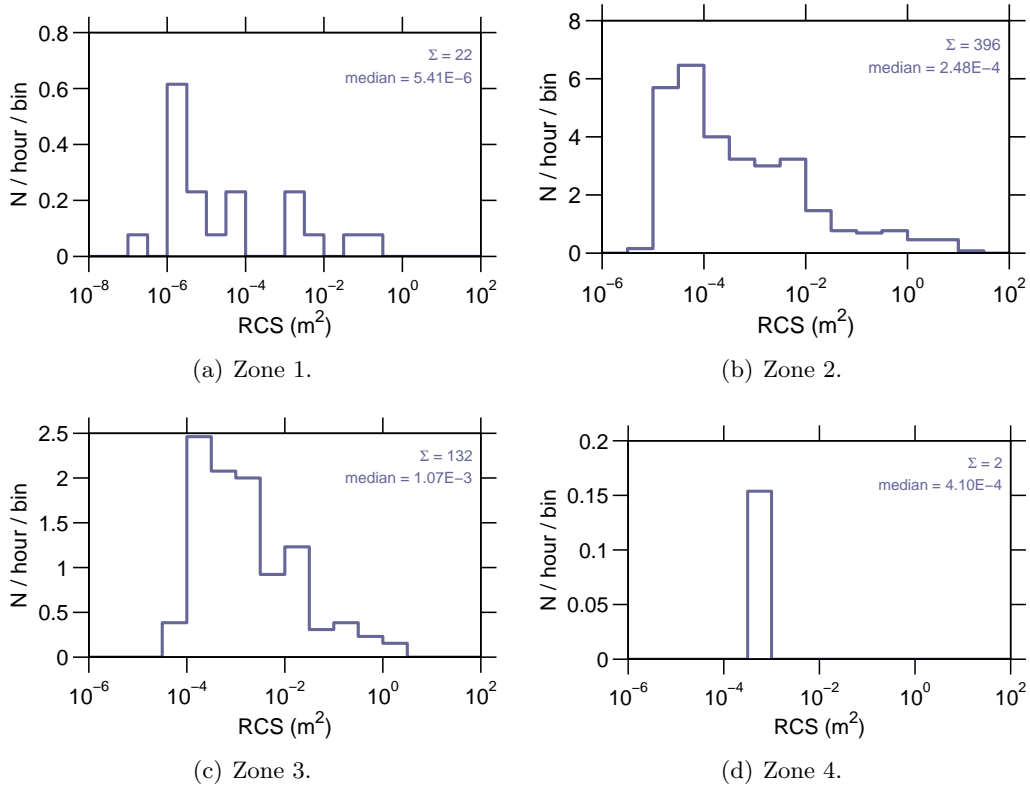
Figure 9: Event rate v RCS on 06-September-2007.
