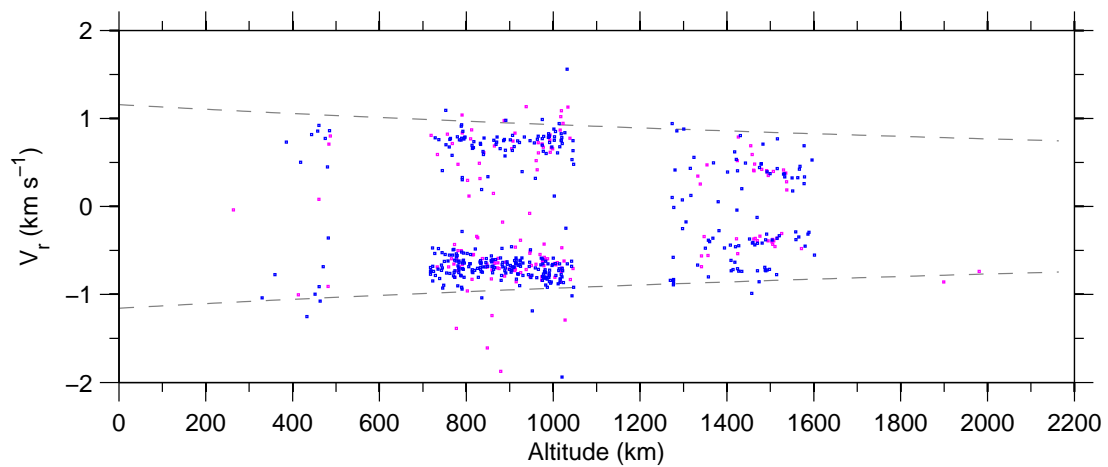
Figure 7: Doppler-velocity v altitude on 06-September-2007.
