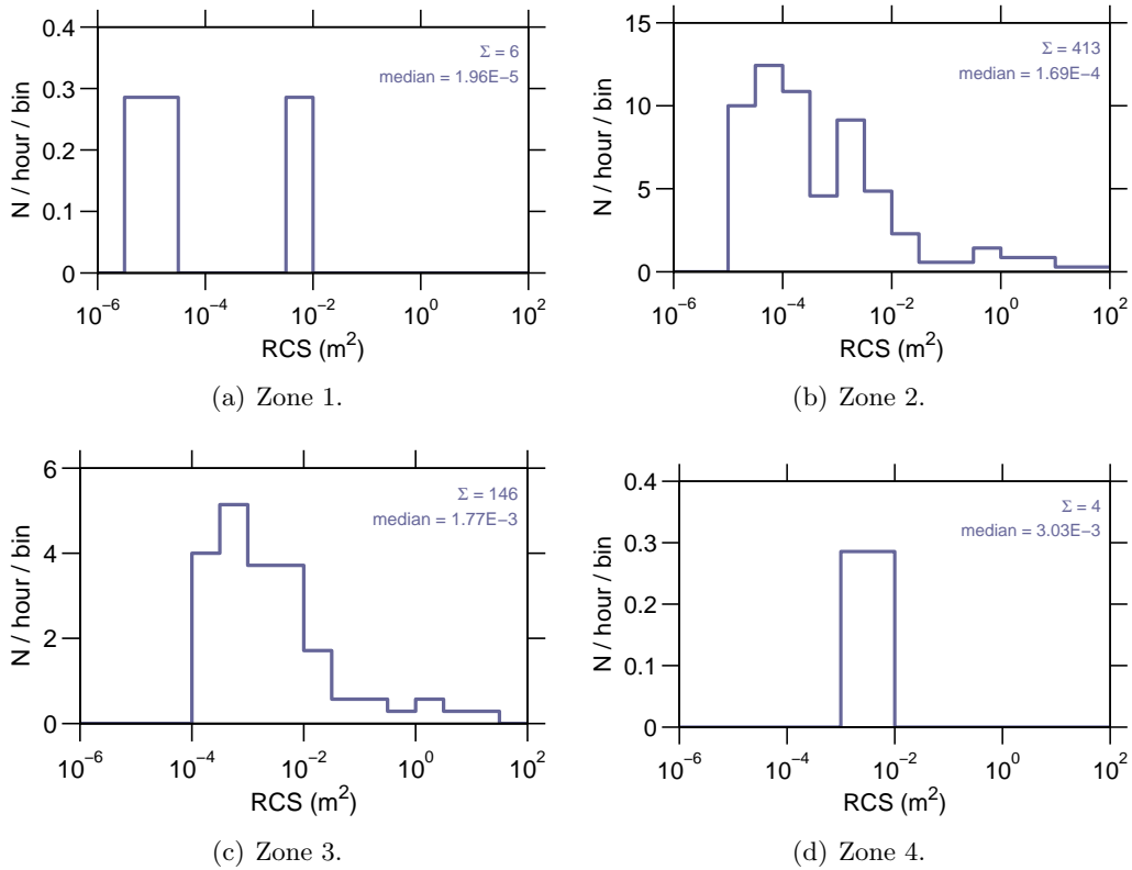
Figure 9: Event rate v RCS on 05-September-2007.
