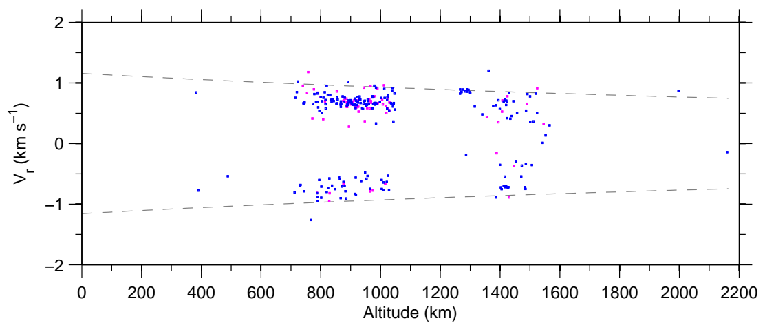
Figure 7: Doppler-velocity v altitude on 05-September-2007.
