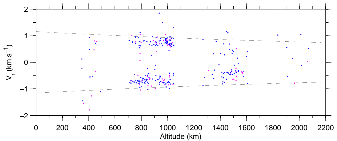
Figure 7: Doppler-velocity v altitude on 04-September-2007.
