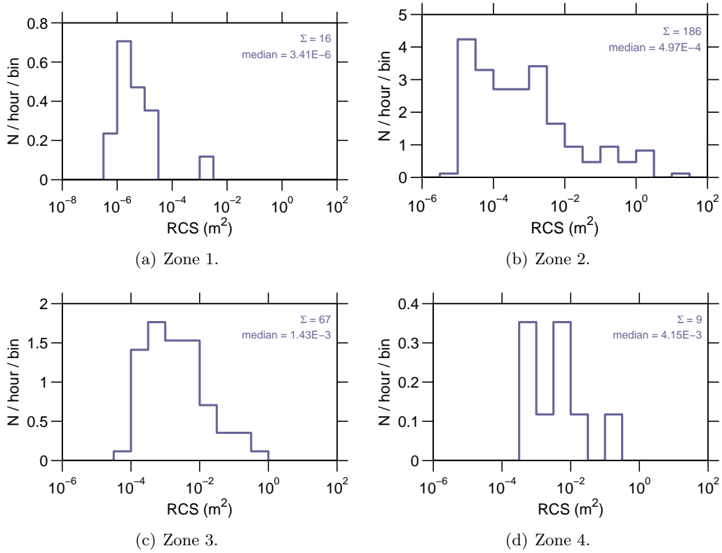
Figure 9: Event rate v RCS on 04-September-2007.
