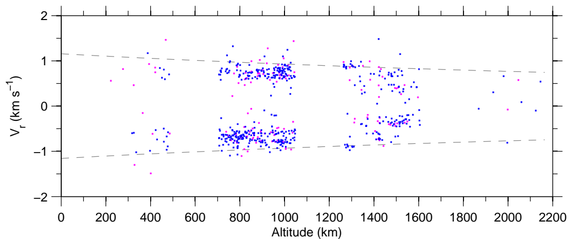
Figure 7: Doppler-velocity v altitude on 19-August-2007.
