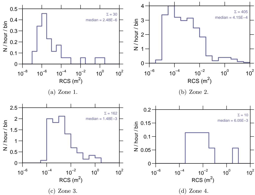
Figure 9: Event rate v RCS on 19-August-2007.
