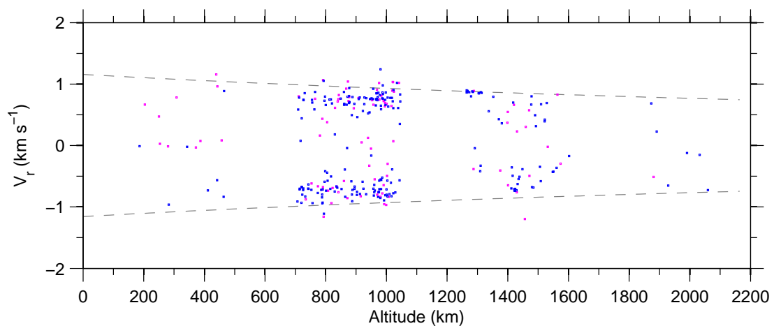
Figure 7: Doppler-velocity v altitude on 14-August-2007.
