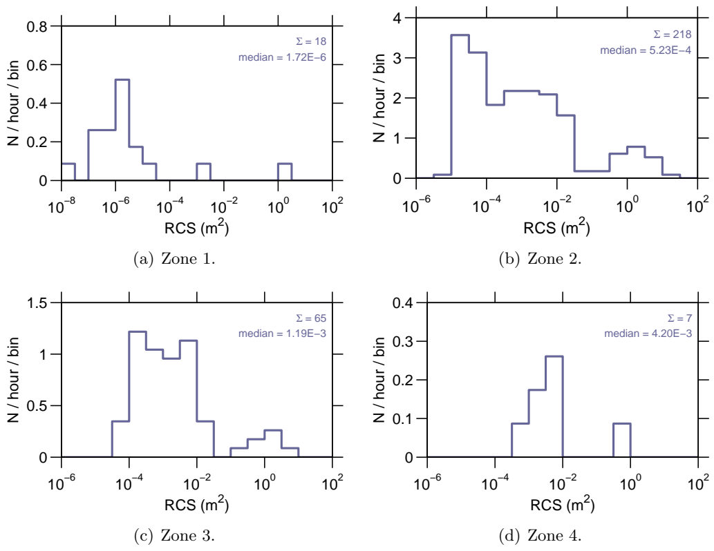
Figure 9: Event rate v RCS on 14-August-2007.
