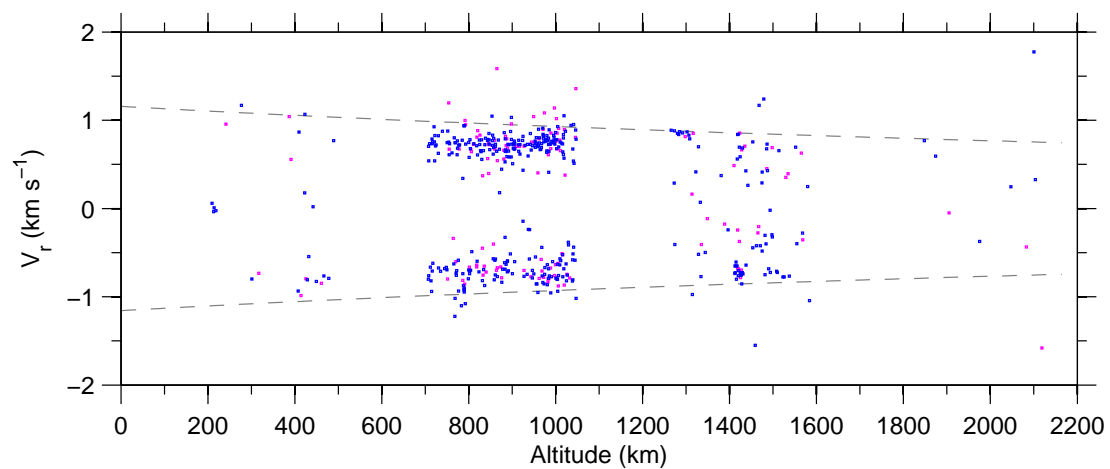
Figure 7: Doppler-velocity v altitude on 07-August-2007.
