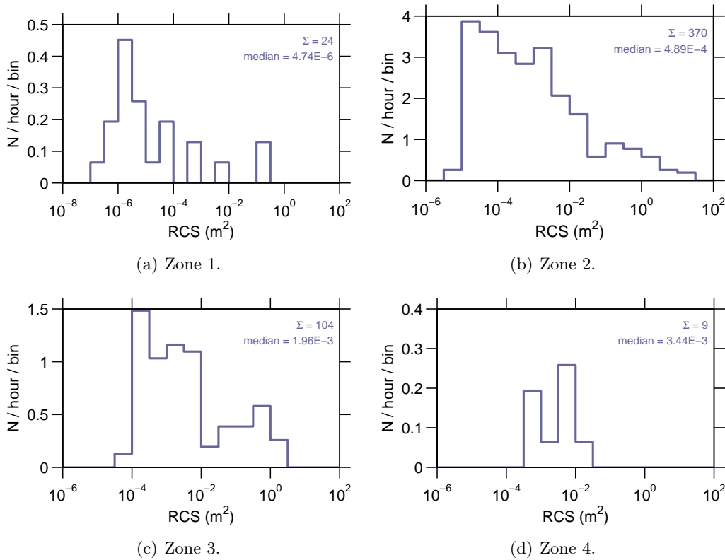
Figure 9: Event rate v RCS on 07-August-2007.
