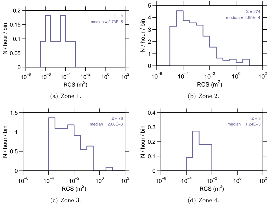
Figure 9: Event rate v RCS on 23-May-2007.
