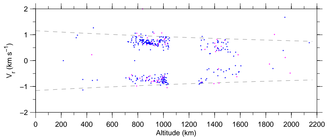
Figure 7: Doppler-velocity v altitude on 23-May-2007.
