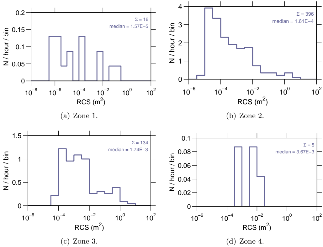
Figure 9: Event rate v RCS on 02-May-2007.
