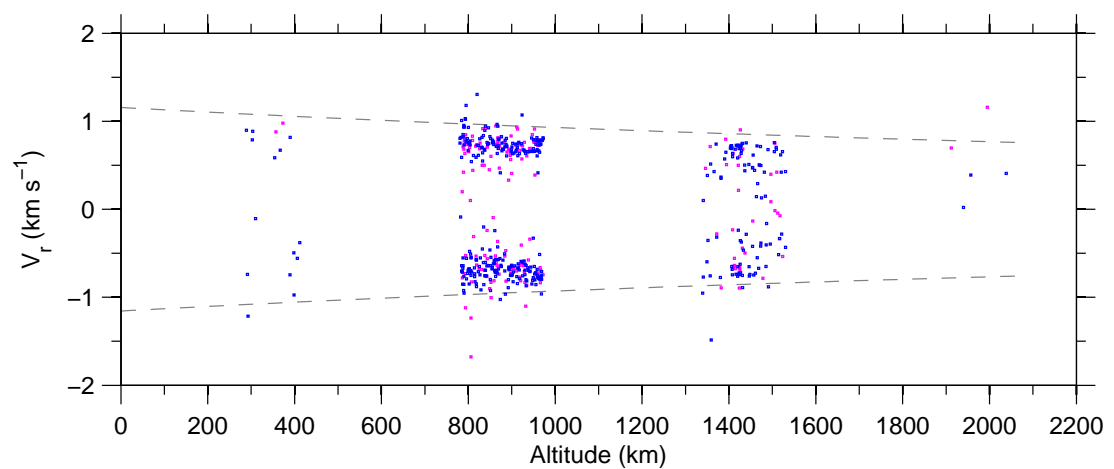
Figure 7: Doppler-velocity v altitude on 02-May-2007.
